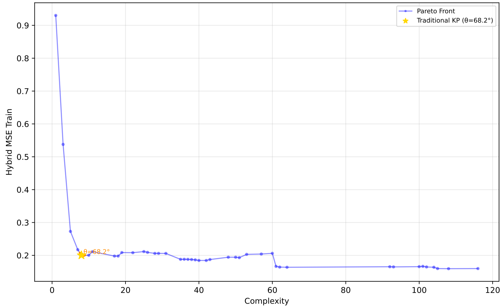
519_vinnie - Run 19 - SVP - Hybrid MSE Train \lambda_1=1.00, \lambda_2=1.00, \lambda_3=1.00 | Difficulty: 0.46 | Method: mckp
