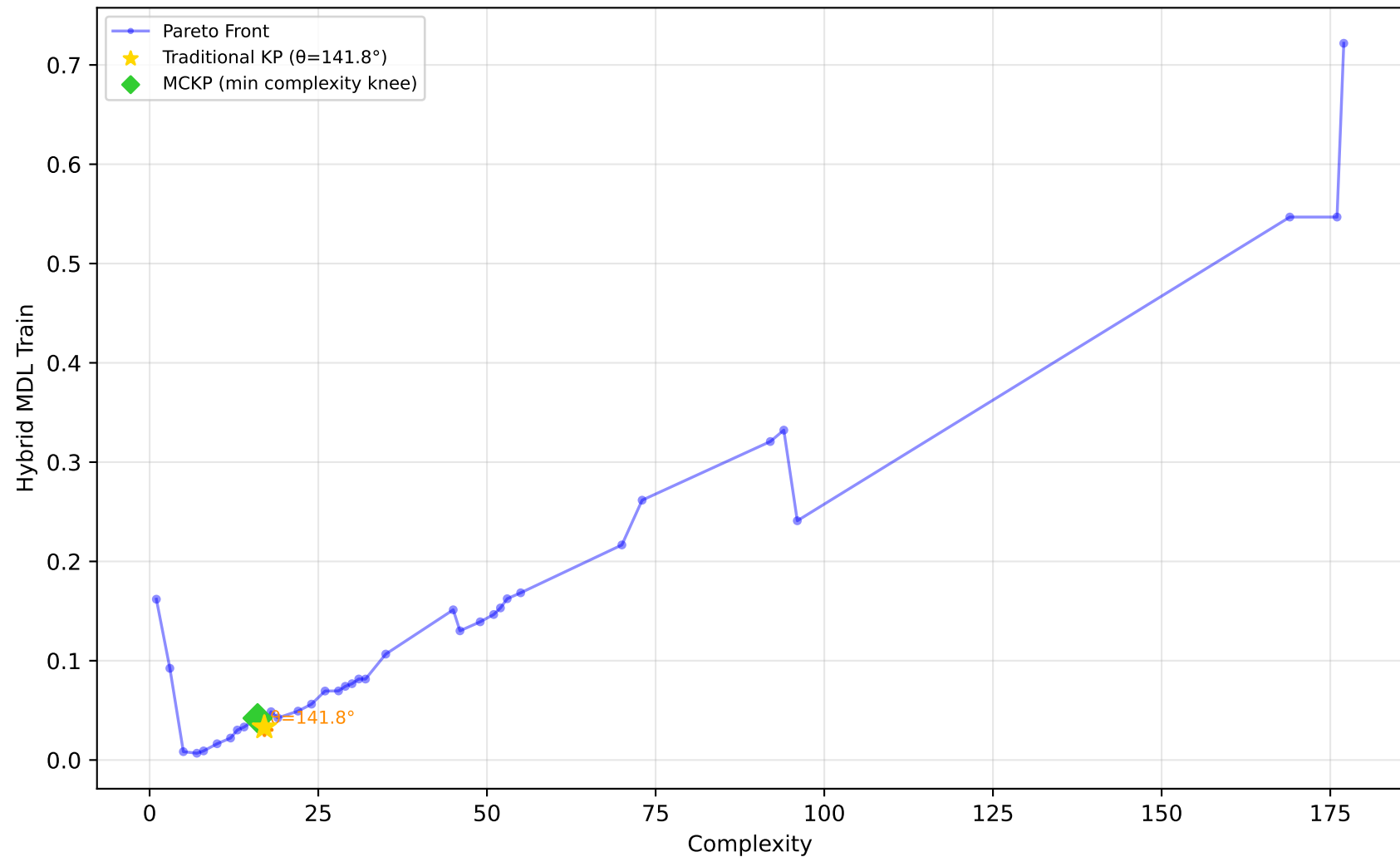
519_vinnie - Run 1 - MVP - Hybrid MDL Train \lambda_1=0.00, \lambda_2=0.10, \lambda_3=0.00 | Difficulty: 0.59 | Method: mckp
