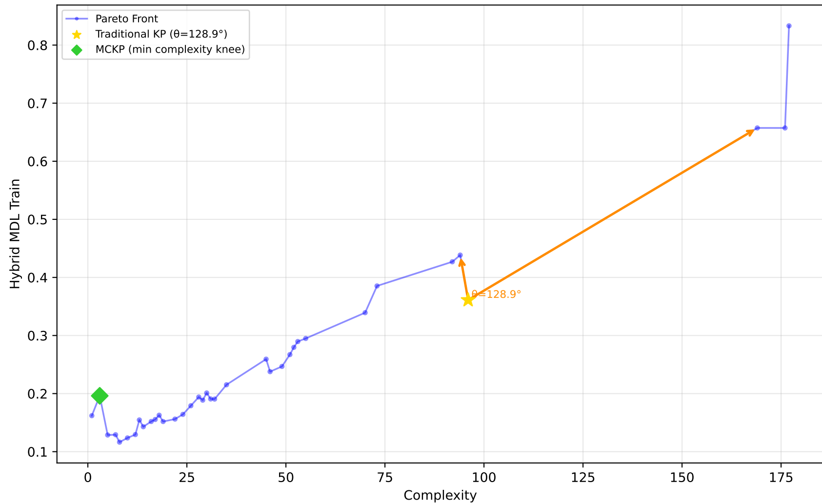
519_vinnie - Run 1 - MVP - Hybrid MDL Train \lambda_1=1.00, \lambda_2=0.00, \lambda_3=1.00 | Difficulty: 0.59 | Method: mckp
