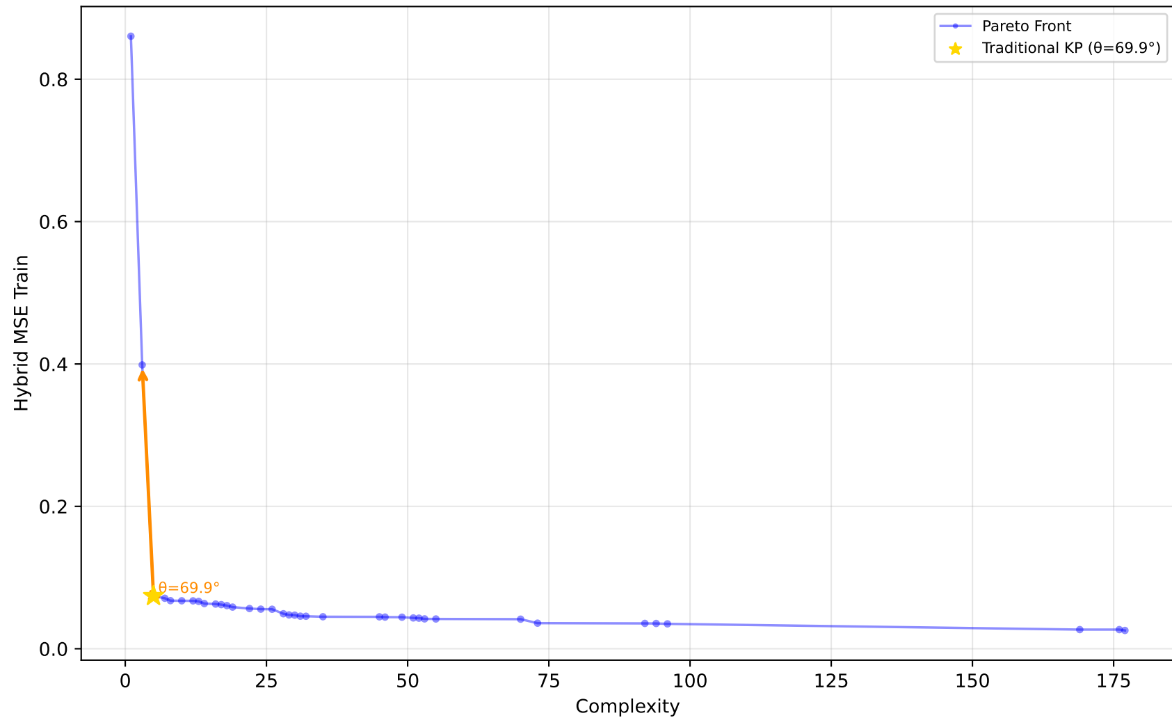
519_vinnie - Run 1 - MVP - Hybrid MSE Train \lambda_1=0.00, \lambda_2=0.10, \lambda_3=0.00 | Difficulty: 0.59 | Method: mckp
