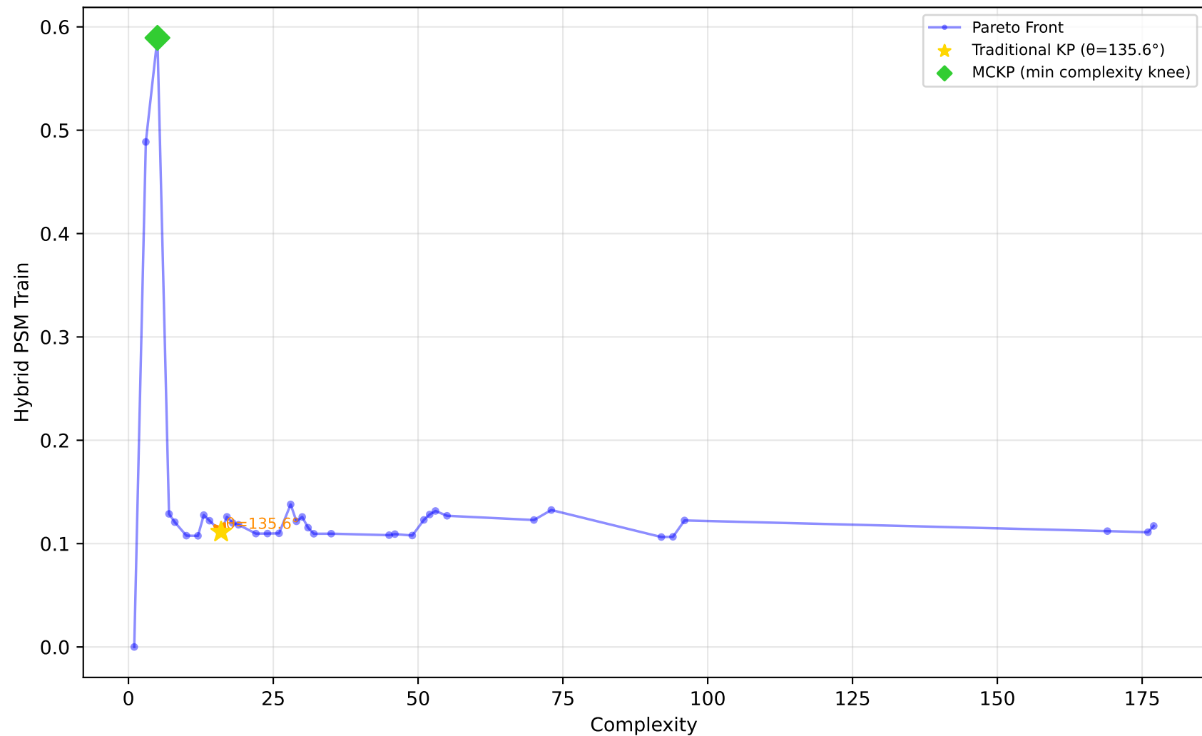
519_vinnie - Run 1 - MVP - Hybrid PSM Train \lambda_1=1.00, \lambda_2=0.00, \lambda_3=1.00 | Difficulty: 0.59 | Method: mckp
