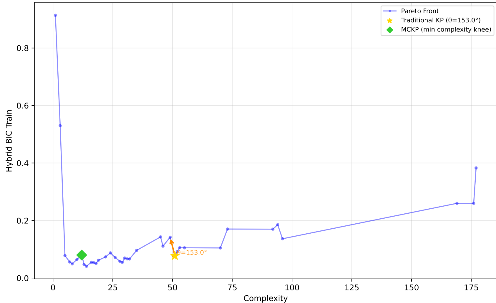
519_vinnie - Run 1 - SVP - Hybrid BIC Train \lambda_1=0.00, \lambda_2=0.00, \lambda_3=0.00 | Difficulty: 0.59 | Method: mckp
