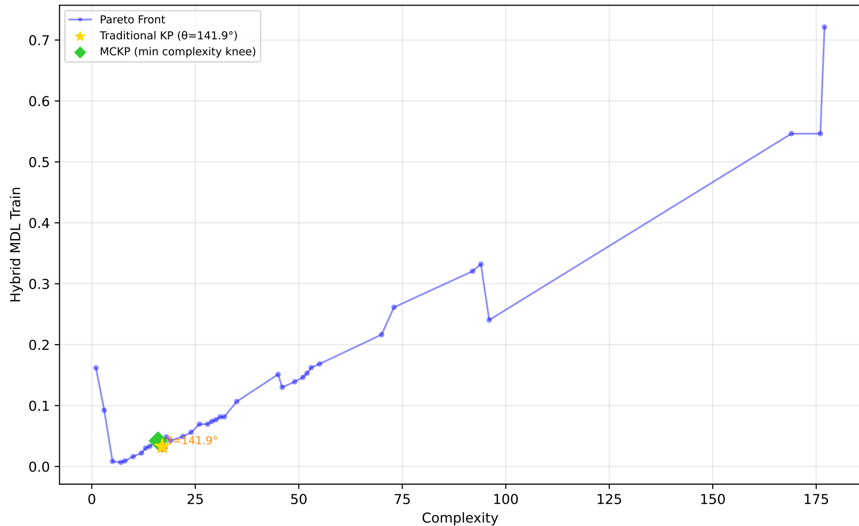
519_vinnie - Run 1 - SVP - Hybrid MDL Train \lambda_1=0.00, \lambda_2=0.00, \lambda_3=0.00 | Difficulty: 0.59 | Method: mckp
