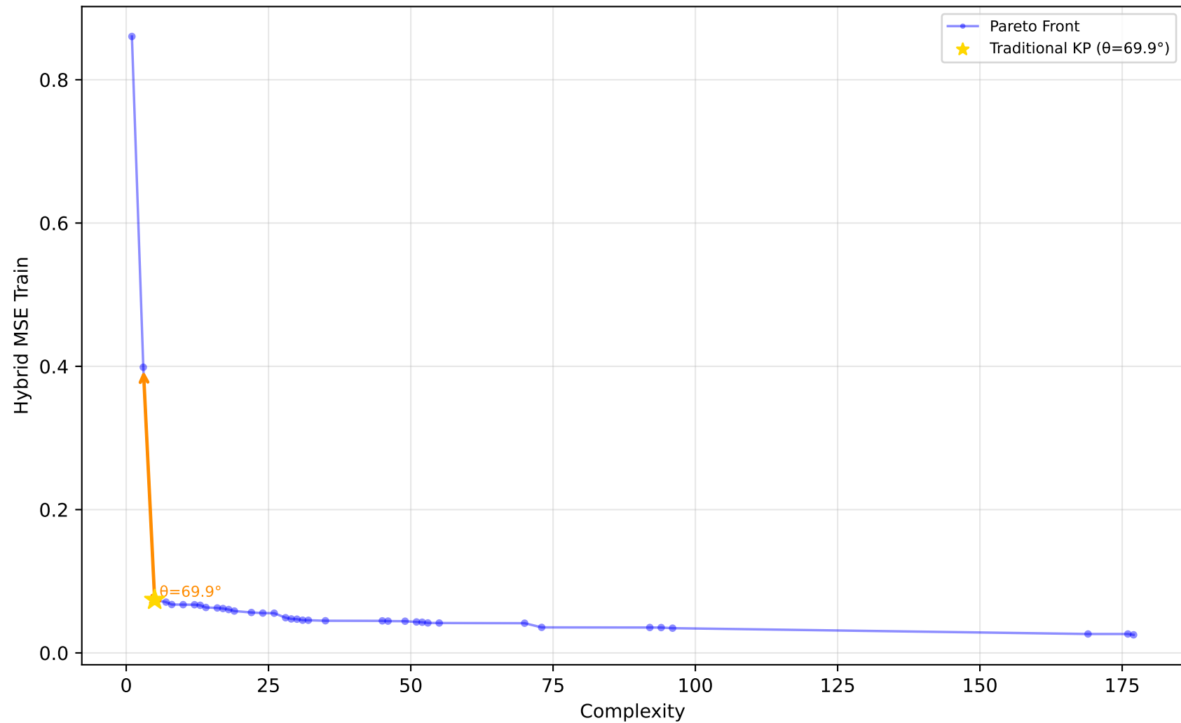
519_vinnie - Run 1 - SVP - Hybrid MSE Train \lambda_1=0.00, \lambda_2=0.00, \lambda_3=0.00 | Difficulty: 0.59 | Method: mckp
