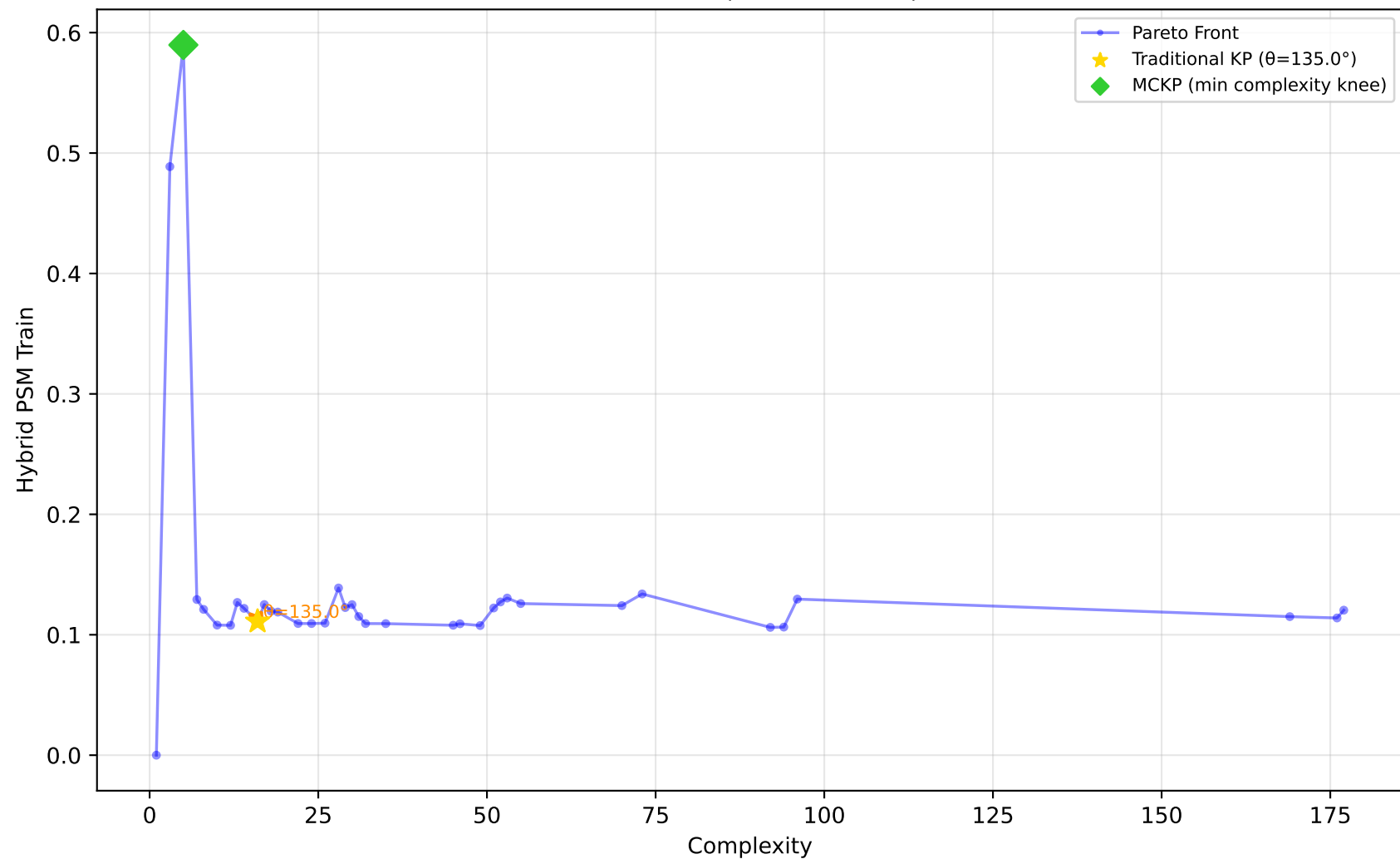
519_vinnie - Run 1 - SVP - Hybrid PSM Train \lambda_1=1.00, \lambda_2=1.00, \lambda_3=1.00 | Difficulty: 0.59 | Method: mckp
