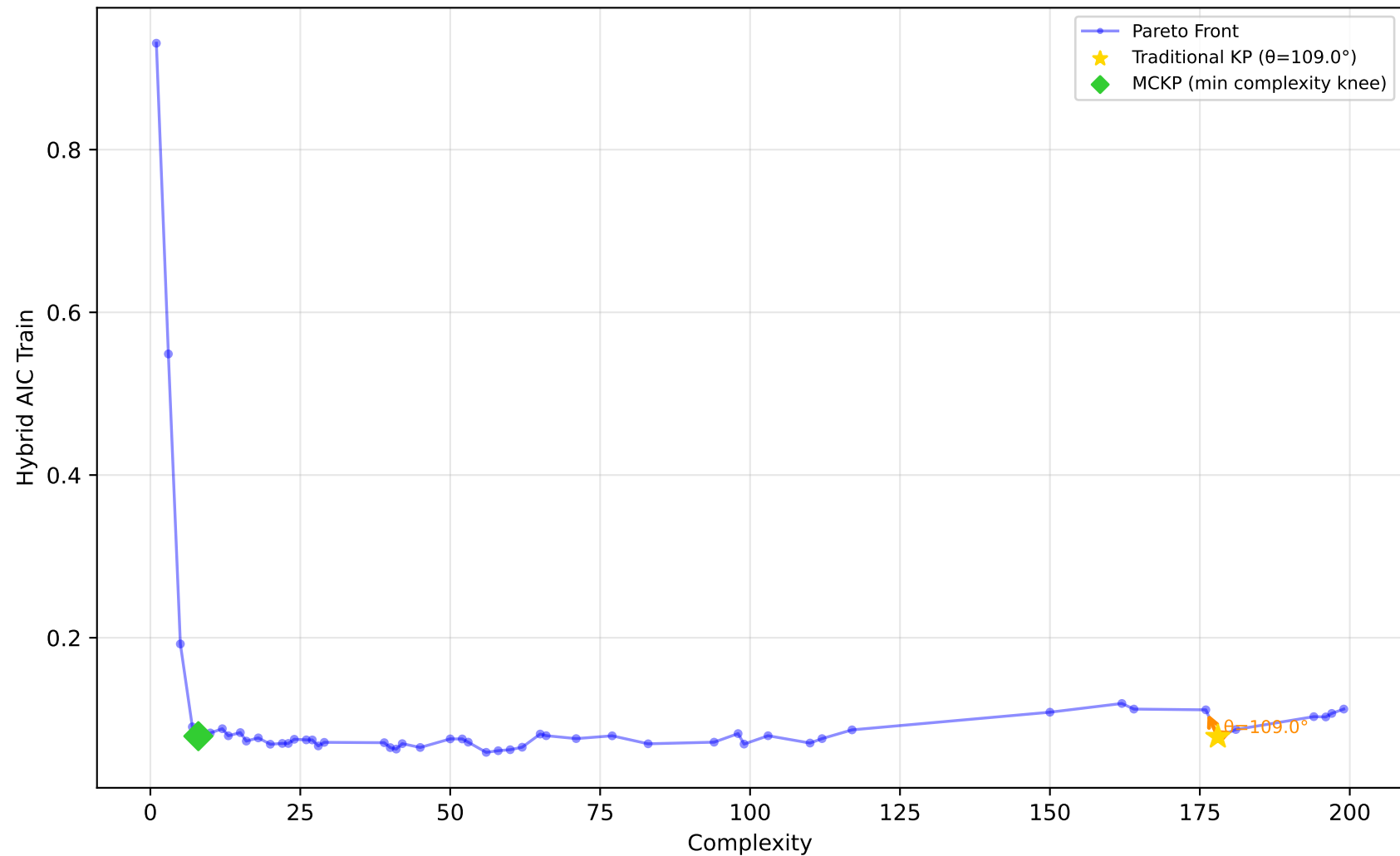
519_vinnie - Run 20 - MVP - Hybrid AIC Train \lambda_1=0.00, \lambda_2=0.10, \lambda_3=0.00 | Difficulty: 0.42 | Method: mckp
