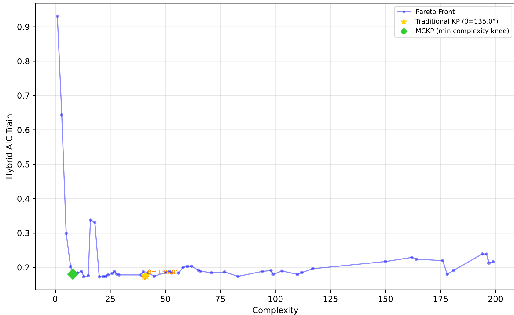
519_vinnie - Run 20 - MVP - Hybrid AIC Train \lambda_1=1.00, \lambda_2=0.00, \lambda_3=1.00 | Difficulty: 0.42 | Method: mckp
