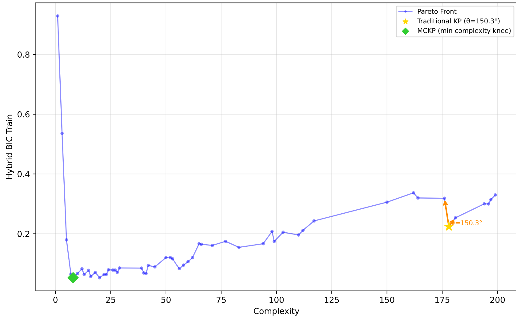
519_vinnie - Run 20 - MVP - Hybrid BIC Train \lambda_1=0.00, \lambda_2=0.10, \lambda_3=0.00 | Difficulty: 0.42 | Method: mckp
