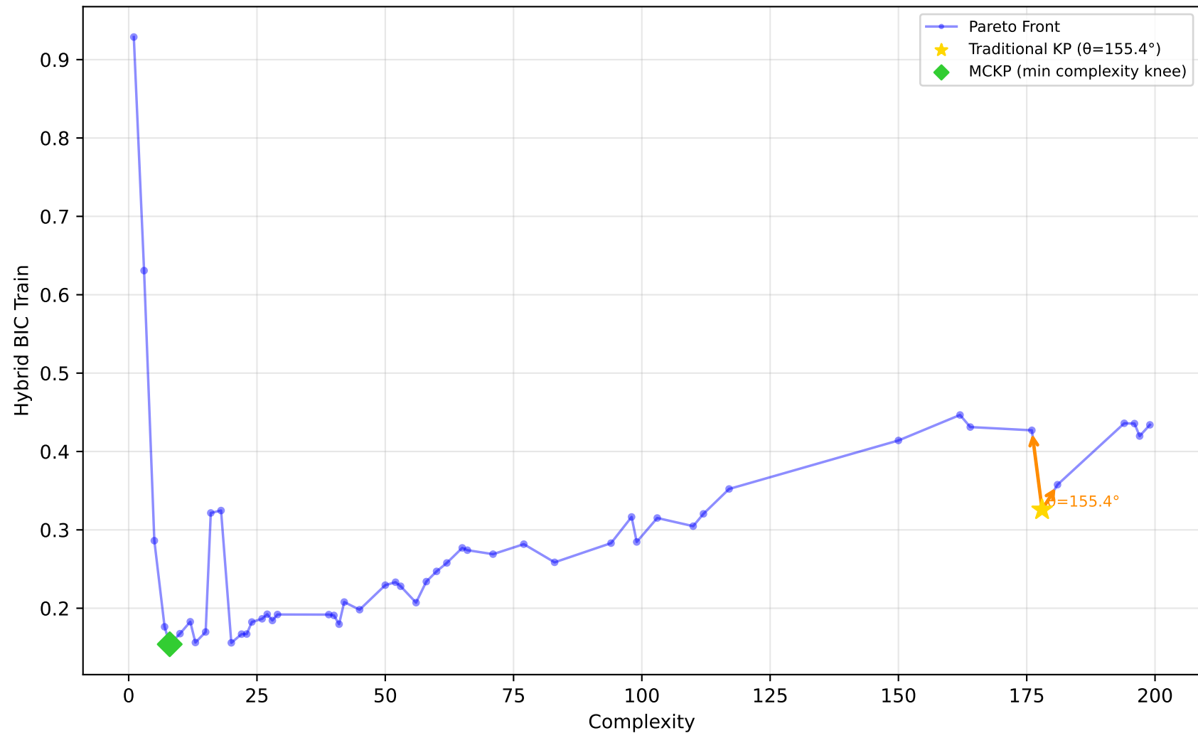
519_vinnie - Run 20 - MVP - Hybrid BIC Train \lambda_1=1.00, \lambda_2=0.00, \lambda_3=1.00 | Difficulty: 0.42 | Method: mckp
