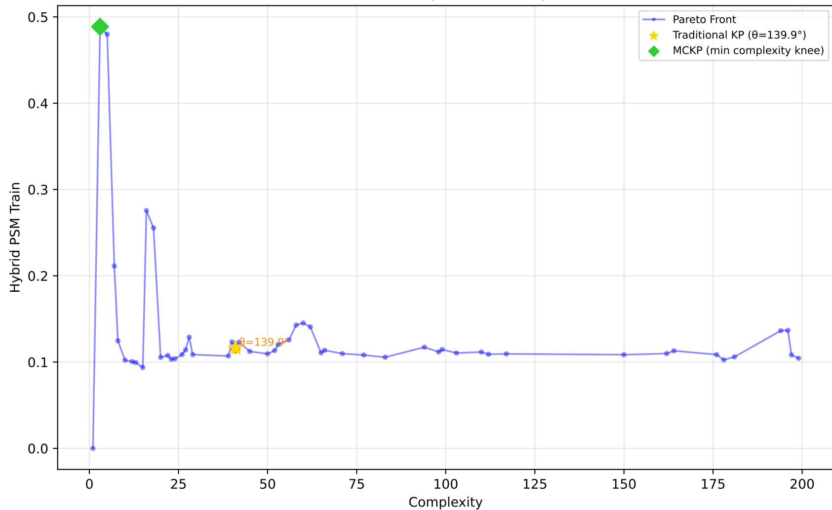
519_vinnie - Run 20 - MVP - Hybrid PSM Train \lambda_1=1.00, \lambda_2=0.00, \lambda_3=1.00 | Difficulty: 0.42 | Method: mckp
