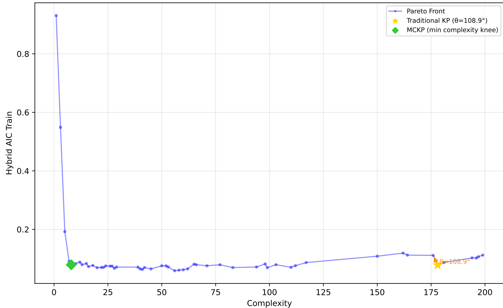
519_vinnie - Run 20 - SVP - Hybrid AIC Train \lambda_1=0.00, \lambda_2=0.00, \lambda_3=0.00 | Difficulty: 0.42 | Method: mckp
