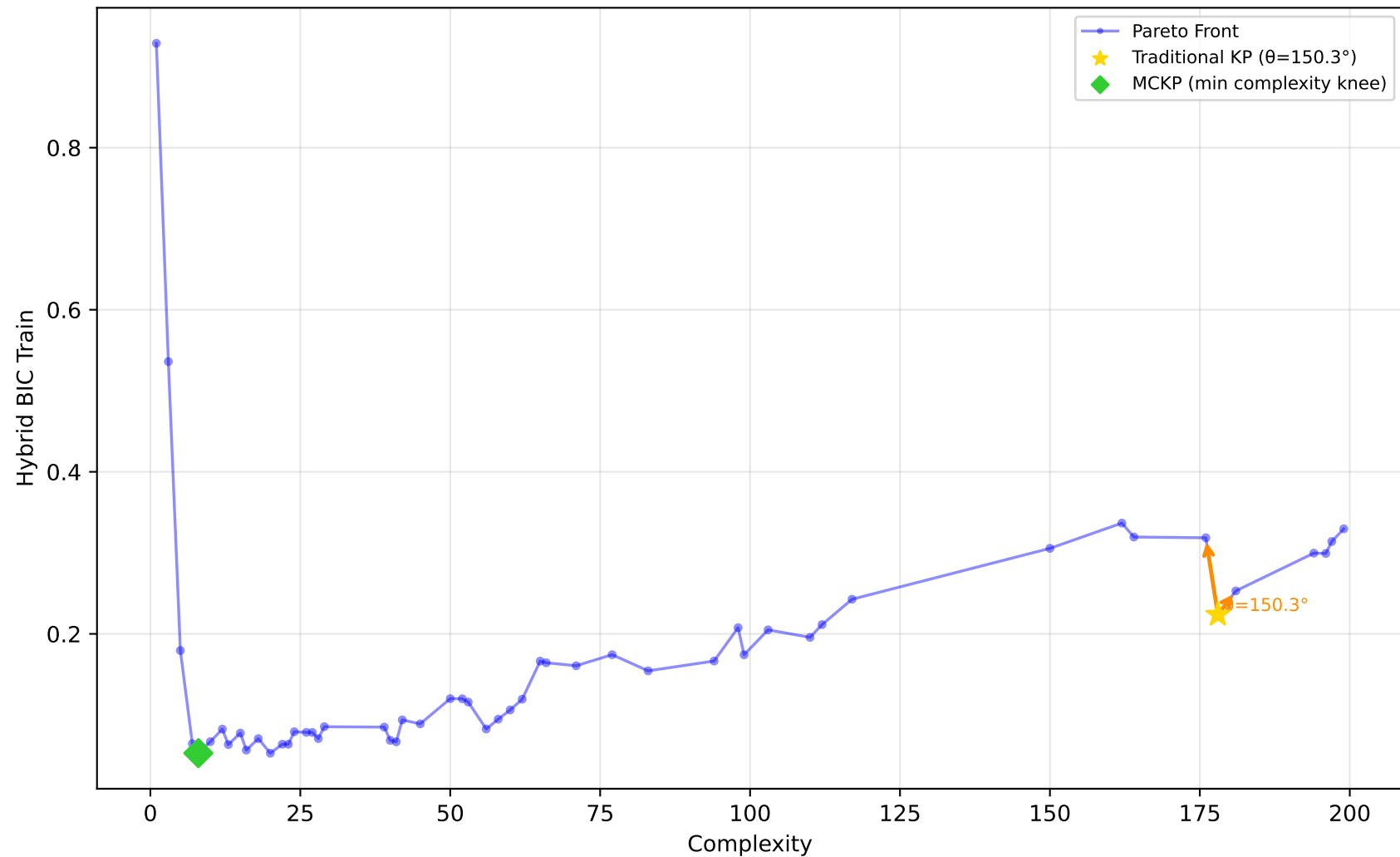
519_vinnie - Run 20 - SVP - Hybrid BIC Train \lambda_1=0.00, \lambda_2=0.00, \lambda_3=0.00 | Difficulty: 0.42 | Method: mckp
