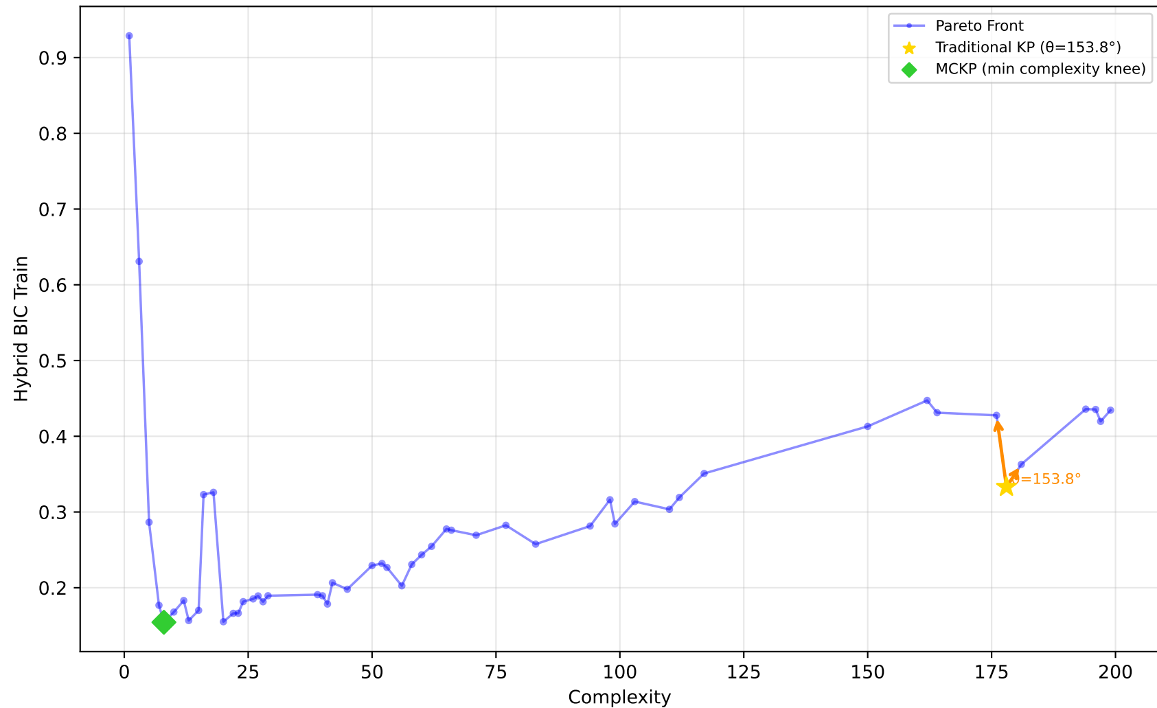
519_vinnie - Run 20 - SVP - Hybrid BIC Train \lambda_1=1.00, \lambda_2=1.00, \lambda_3=1.00 | Difficulty: 0.42 | Method: mckp
