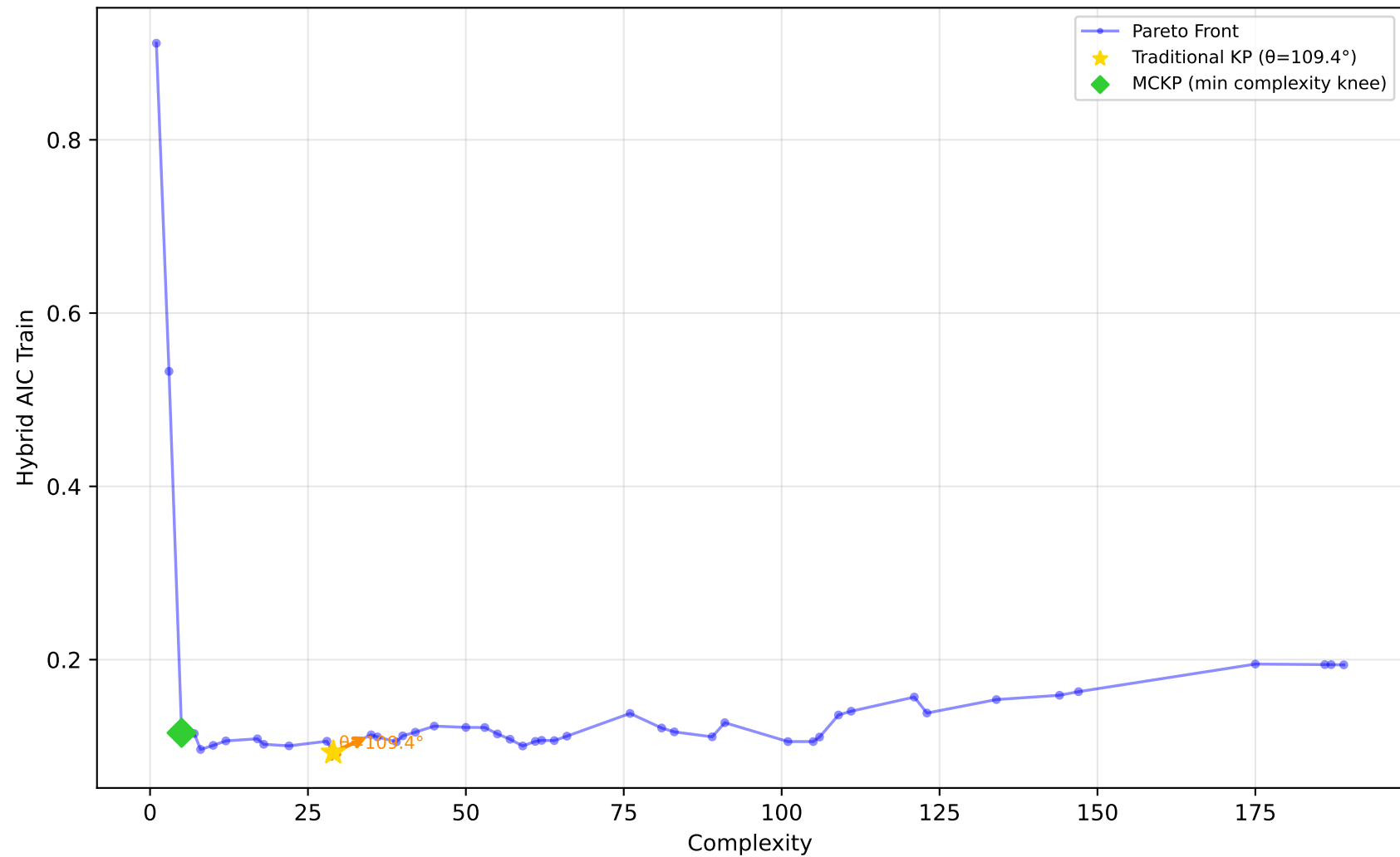
519_vinnie - Run 21 - MVP - Hybrid AIC Train \lambda_1=0.00, \lambda_2=0.10, \lambda_3=0.00 | Difficulty: 0.91 | Method: hmr
