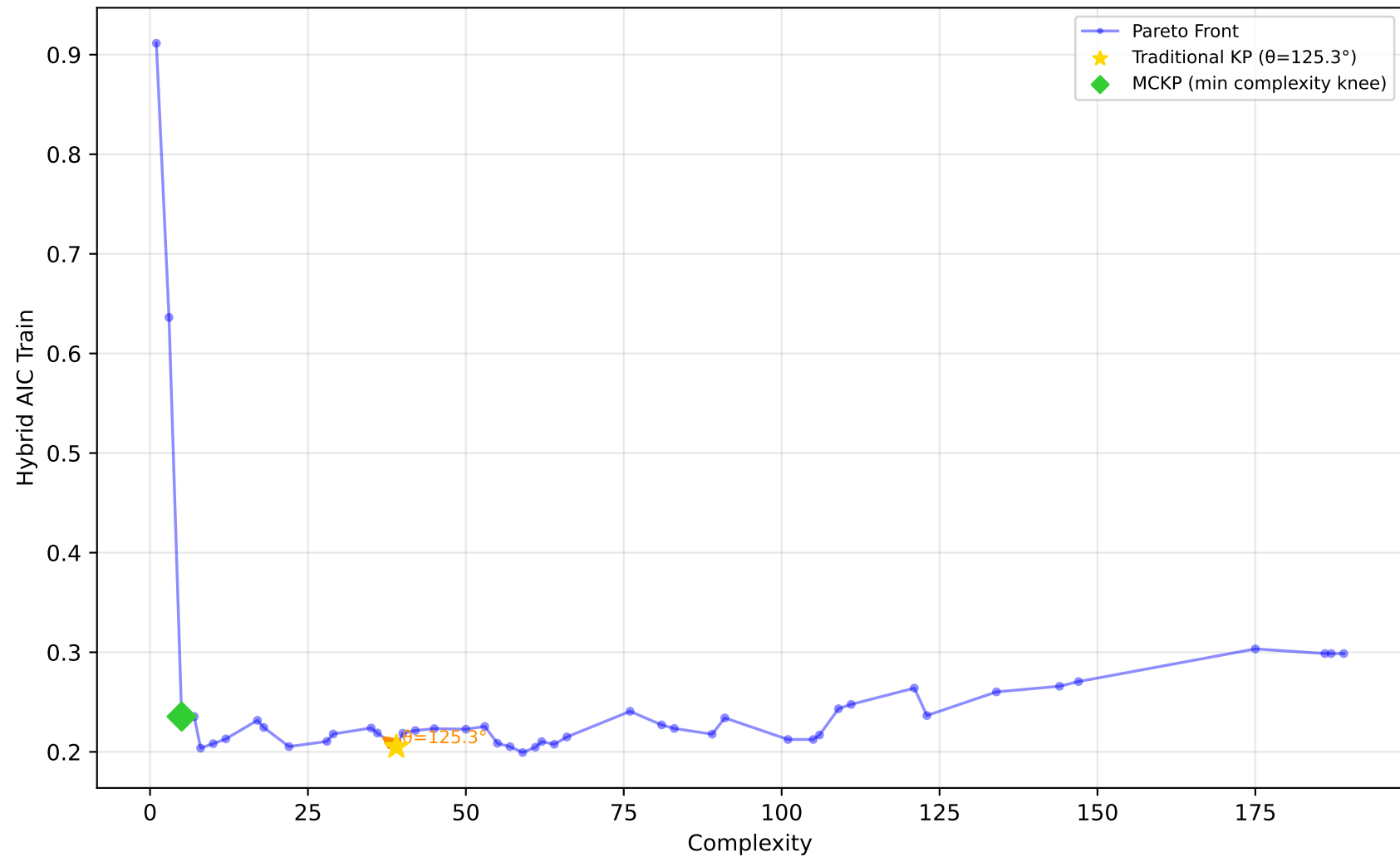
519_vinnie - Run 21 - MVP - Hybrid AIC Train \lambda_1=1.00, \lambda_2=0.00, \lambda_3=1.00 | Difficulty: 0.91 | Method: hmr
