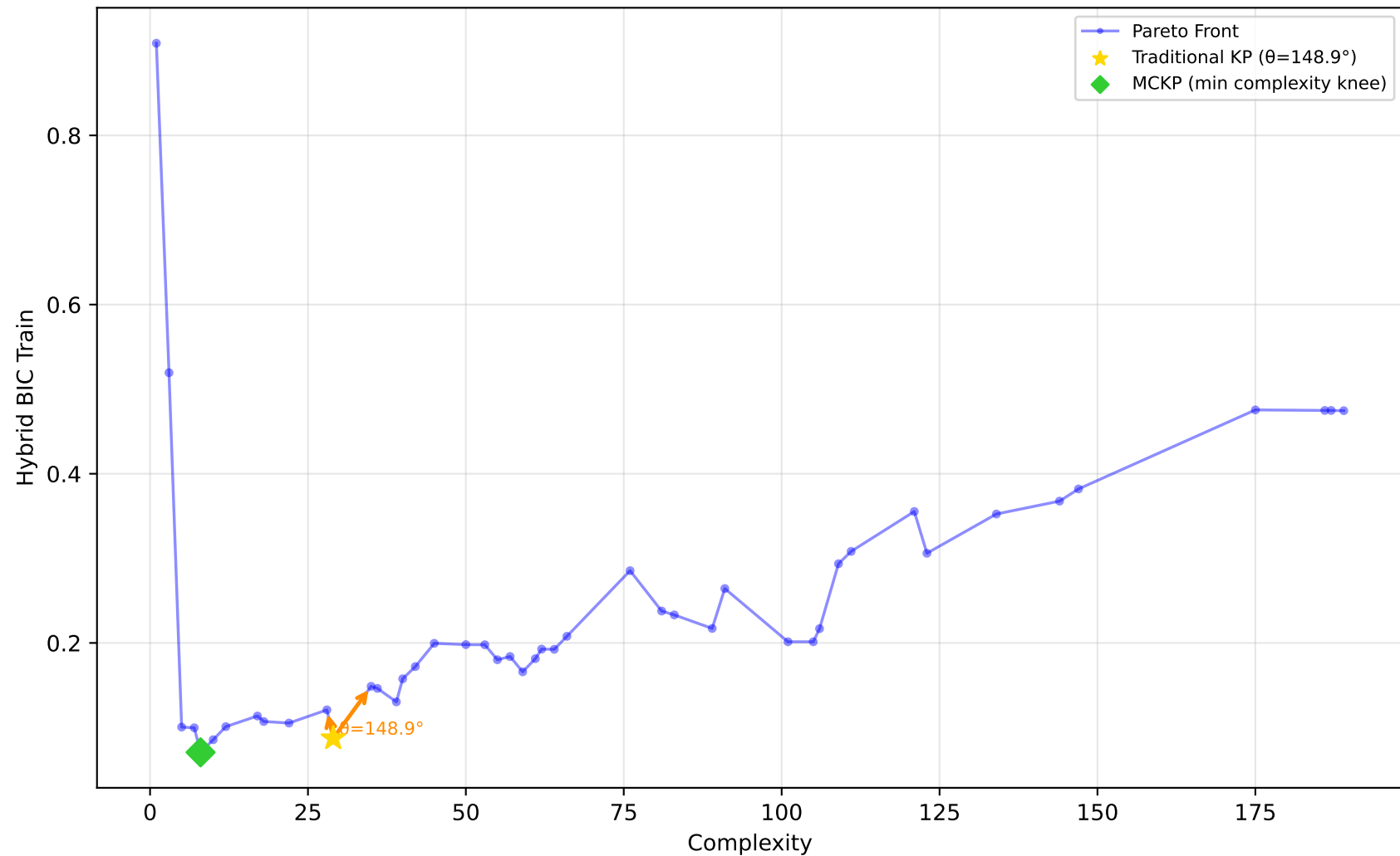
519_vinnie - Run 21 - MVP - Hybrid BIC Train \lambda_1=0.00, \lambda_2=0.10, \lambda_3=0.00 | Difficulty: 0.91 | Method: hmr
