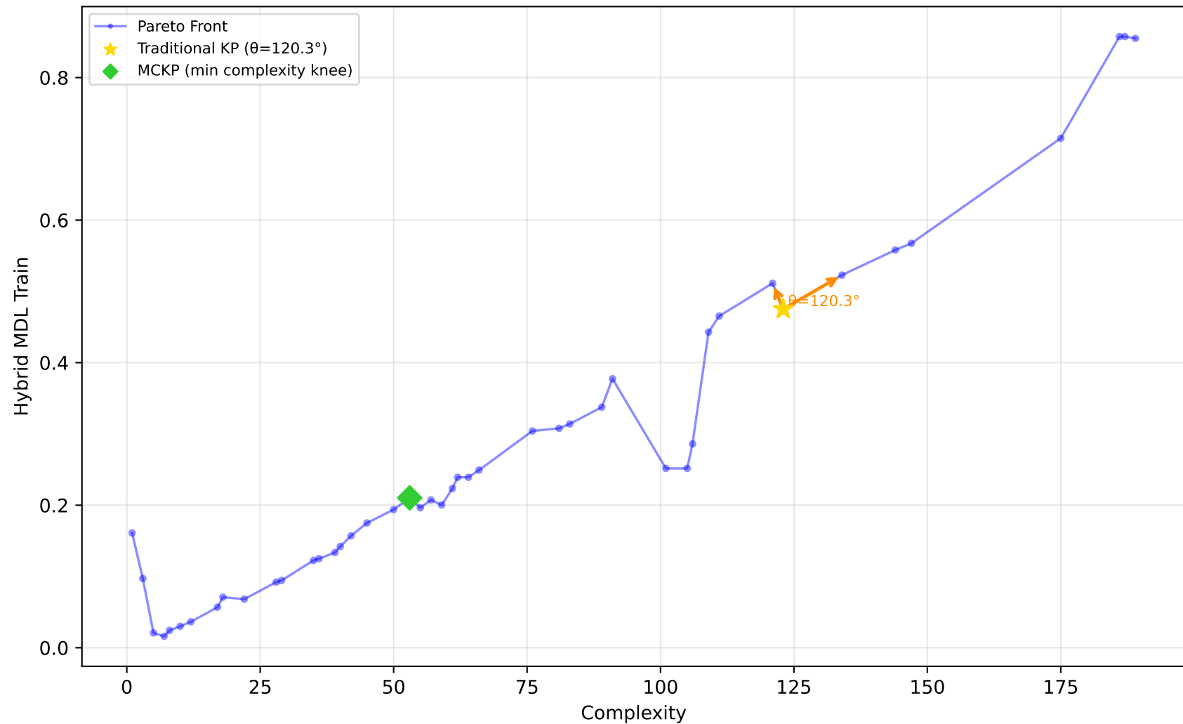
519_vinnie - Run 21 - MVP - Hybrid MDL Train \lambda_1=0.00, \lambda_2=0.10, \lambda_3=0.00 | Difficulty: 0.91 | Method: hmr
