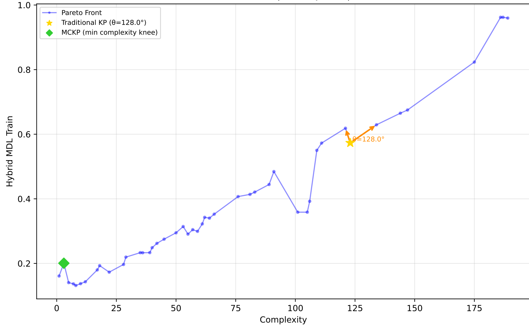
519_vinnie - Run 21 - MVP - Hybrid MDL Train \lambda_1=1.00, \lambda_2=0.00, \lambda_3=1.00 | Difficulty: 0.91 | Method: hmr
