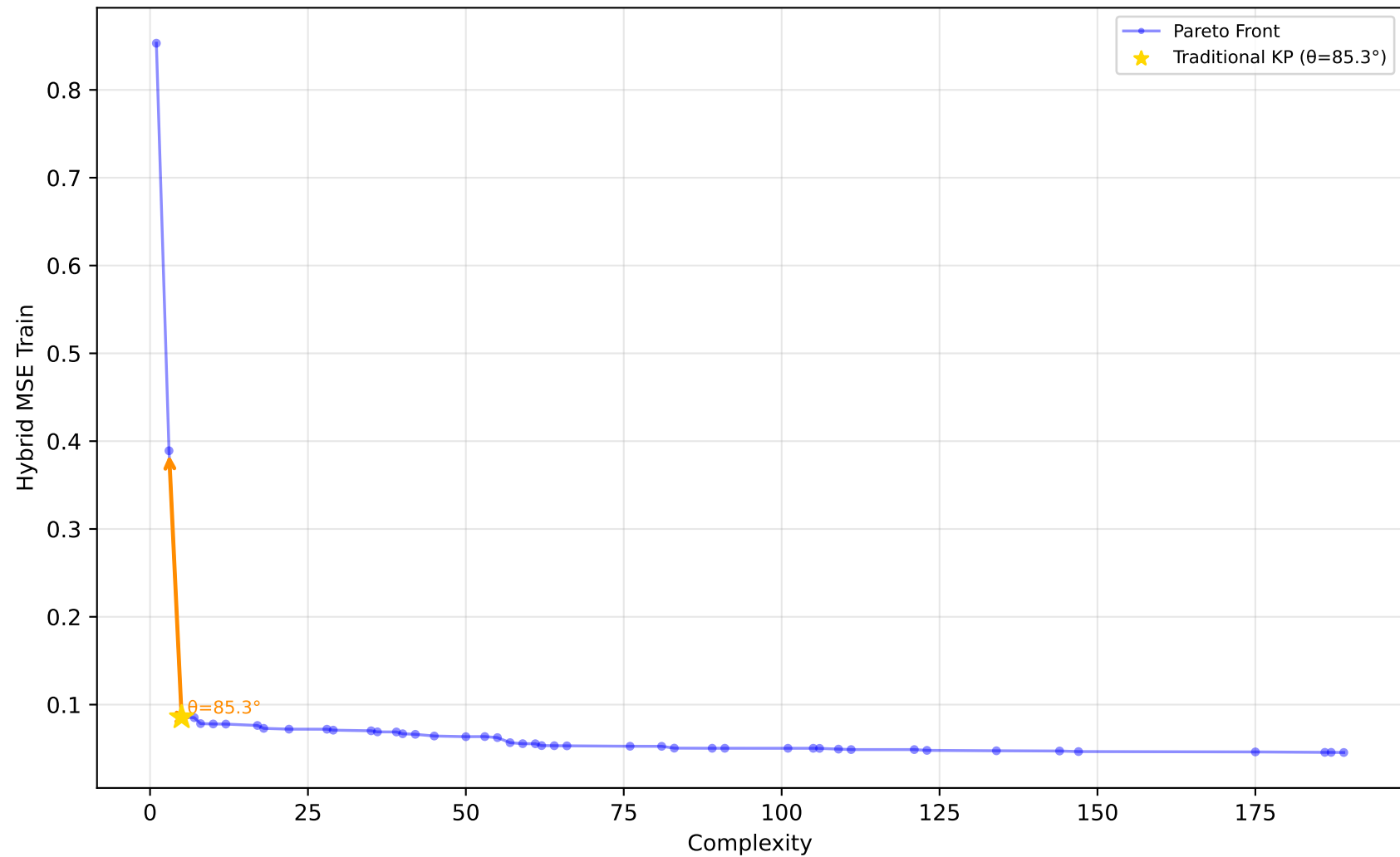
519_vinnie - Run 21 - MVP - Hybrid MSE Train \lambda_1=0.00, \lambda_2=0.10, \lambda_3=0.00 | Difficulty: 0.91 | Method: hmr
