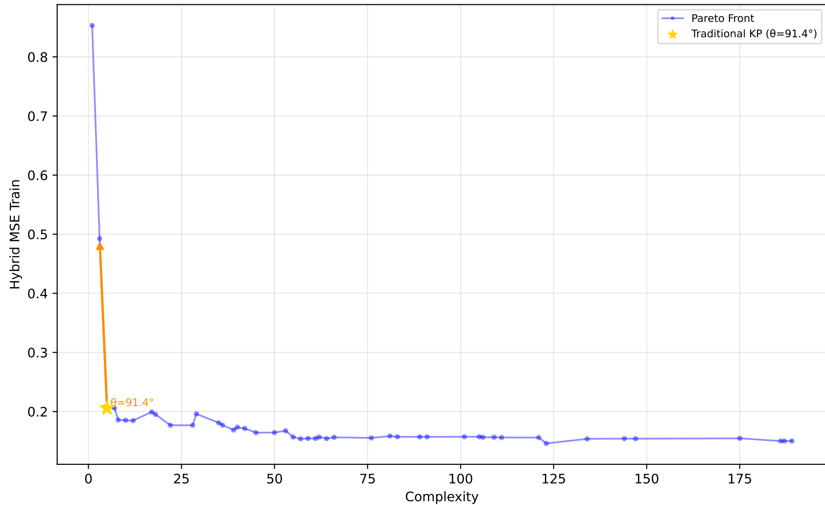
519_vinnie - Run 21 - MVP - Hybrid MSE Train \lambda_1=1.00, \lambda_2=0.00, \lambda_3=1.00 | Difficulty: 0.91 | Method: hmr
