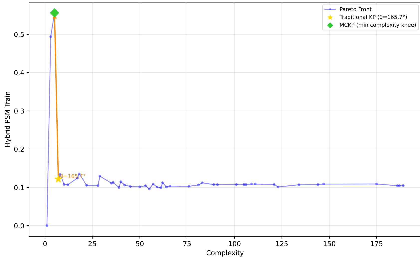
519_vinnie - Run 21 - MVP - Hybrid PSM Train \lambda_1=1.00, \lambda_2=0.00, \lambda_3=1.00 | Difficulty: 0.91 | Method: hmr
