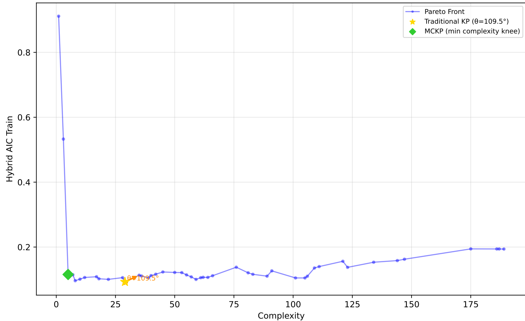
519_vinnie - Run 21 - SVP - Hybrid AIC Train \lambda_1=0.00, \lambda_2=0.00, \lambda_3=0.00 | Difficulty: 0.91 | Method: hmr
