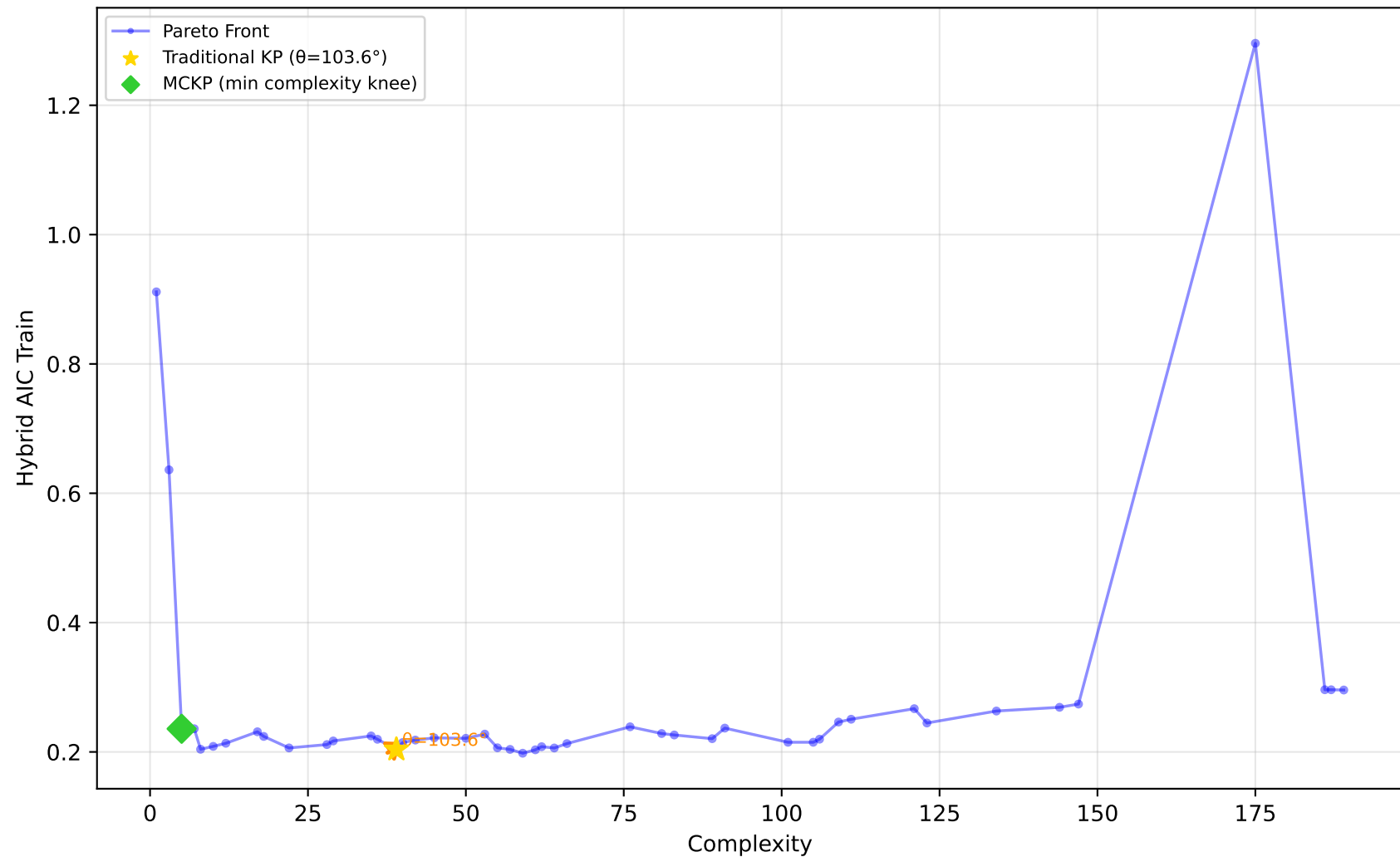
519_vinnie - Run 21 - SVP - Hybrid AIC Train \lambda_1=1.00, \lambda_2=1.00, \lambda_3=1.00 | Difficulty: 0.91 | Method: hmr
