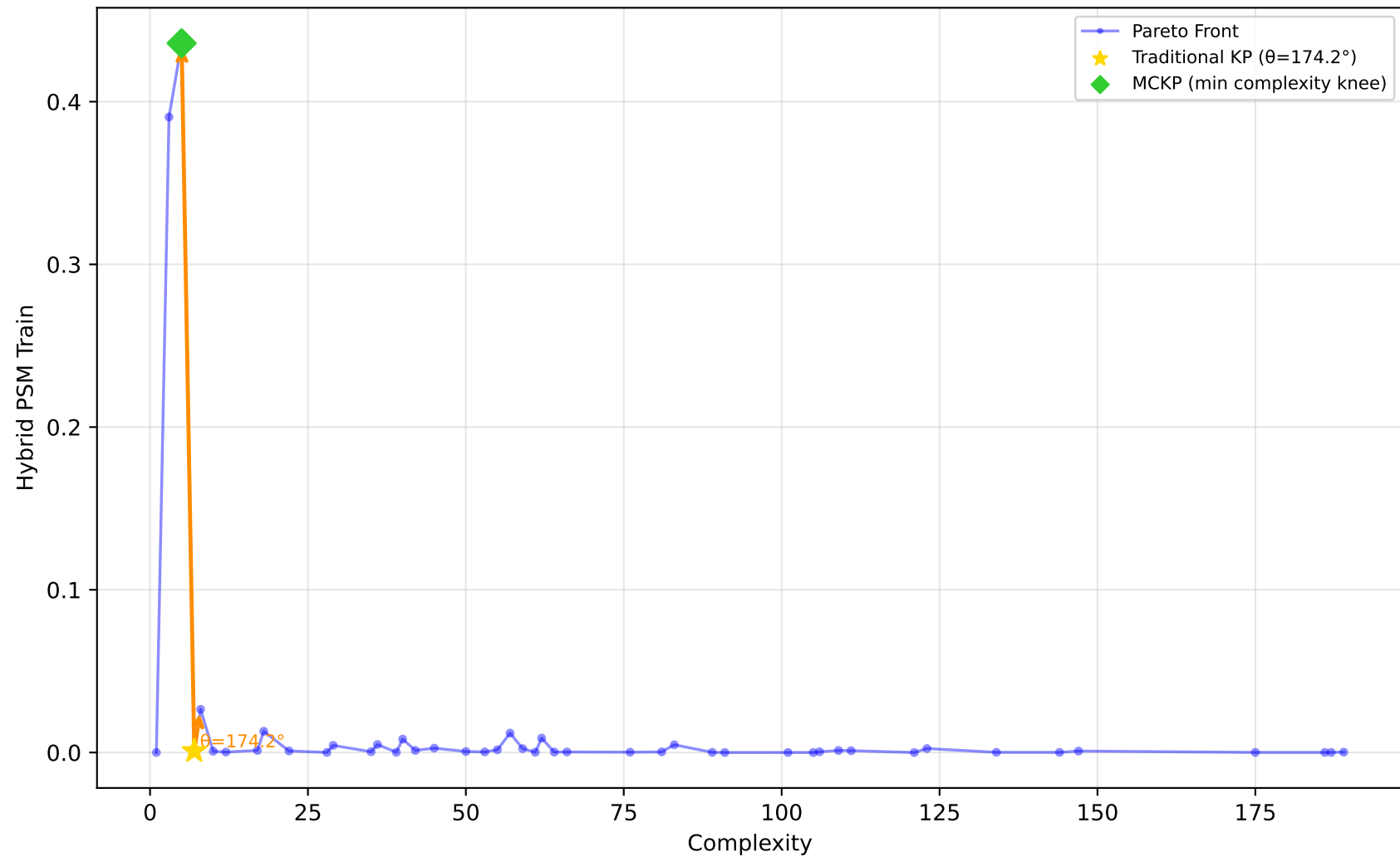
519_vinnie - Run 21 - SVP - Hybrid PSM Train \lambda_1=0.00, \lambda_2=0.00, \lambda_3=0.00 | Difficulty: 0.91 | Method: hmr
