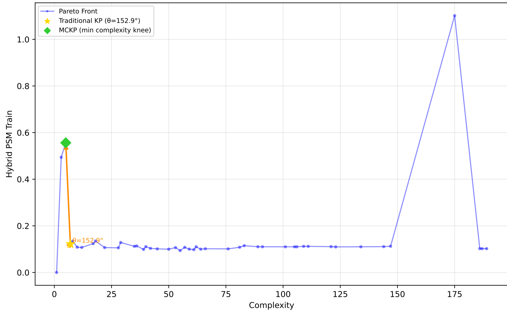
519_vinnie - Run 21 - SVP - Hybrid PSM Train \lambda_1=1.00, \lambda_2=1.00, \lambda_3=1.00 | Difficulty: 0.91 | Method: hmr
