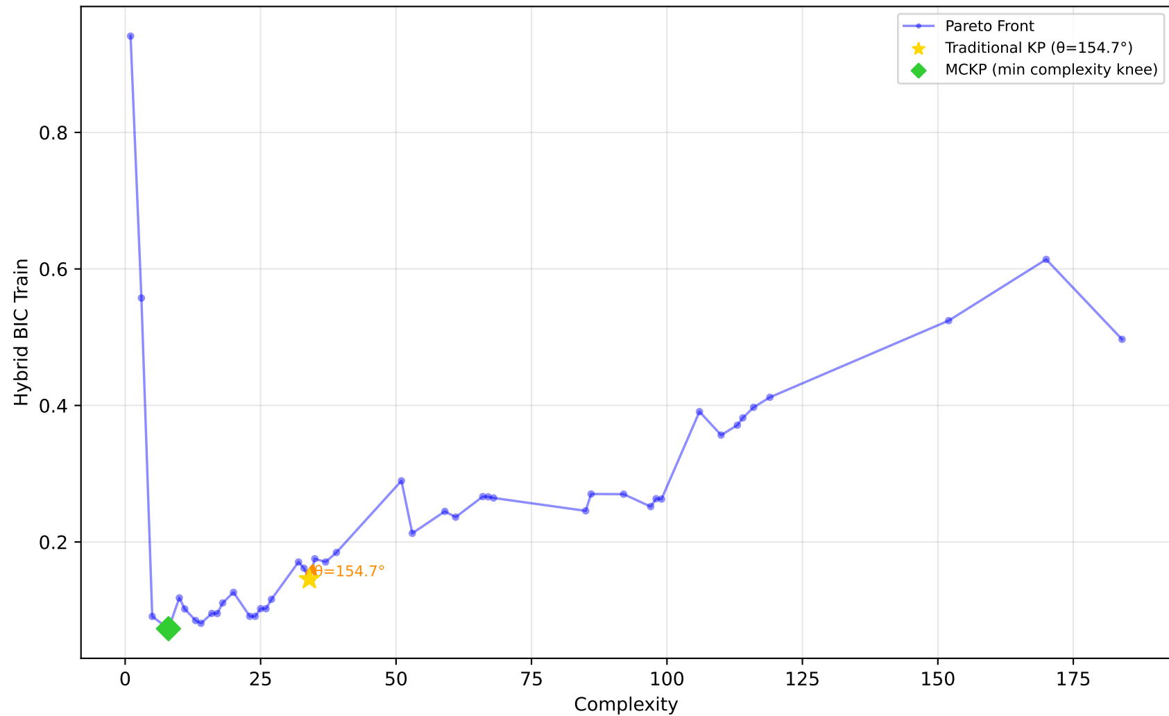
519_vinnie - Run 22 - MVP - Hybrid BIC Train \lambda_1=0.00, \lambda_2=0.10, \lambda_3=0.00 | Difficulty: 0.95 | Method: hmr
