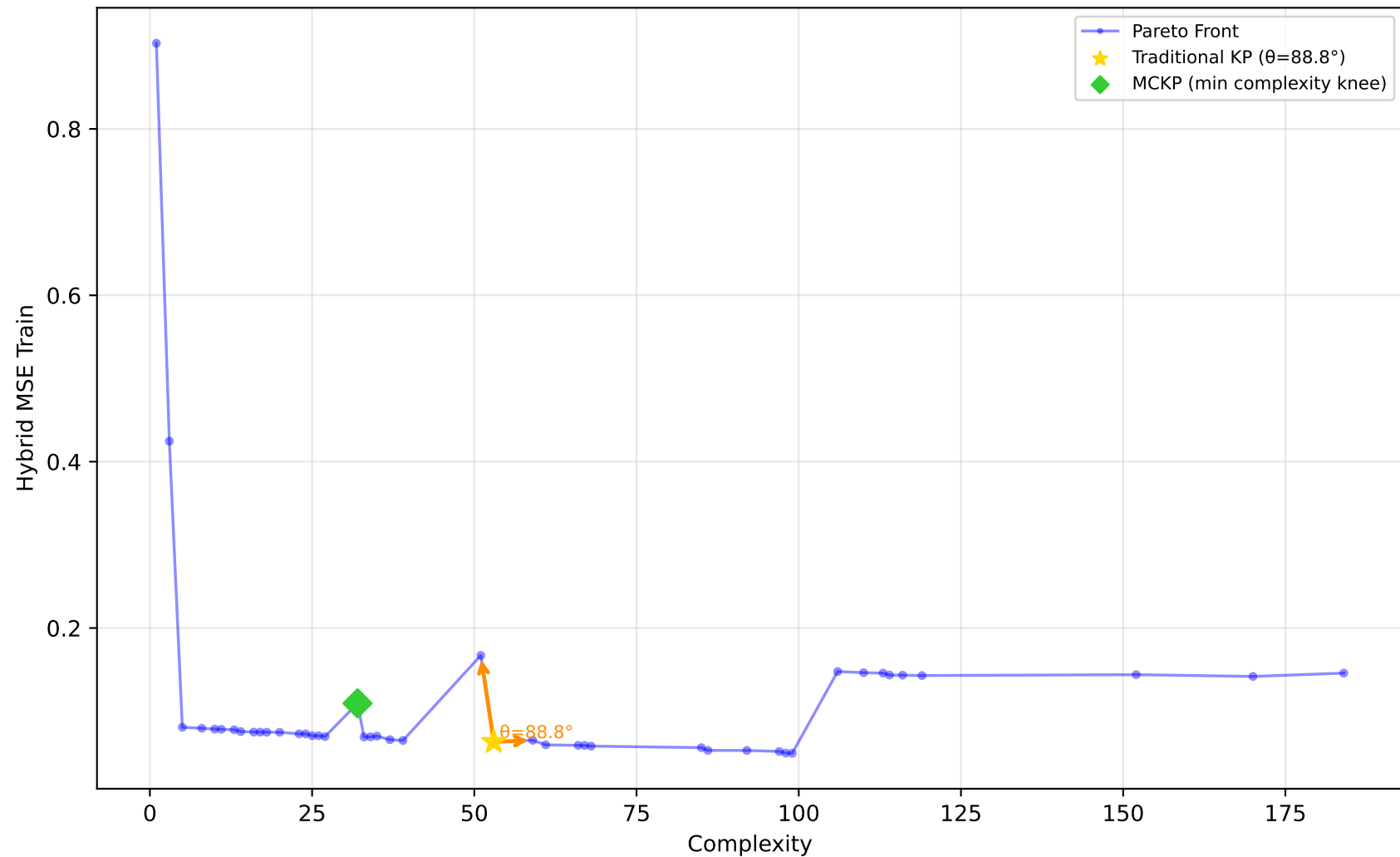
519_vinnie - Run 22 - MVP - Hybrid MSE Train \lambda_1=0.00, \lambda_2=0.10, \lambda_3=0.00 | Difficulty: 0.95 | Method: hmr
