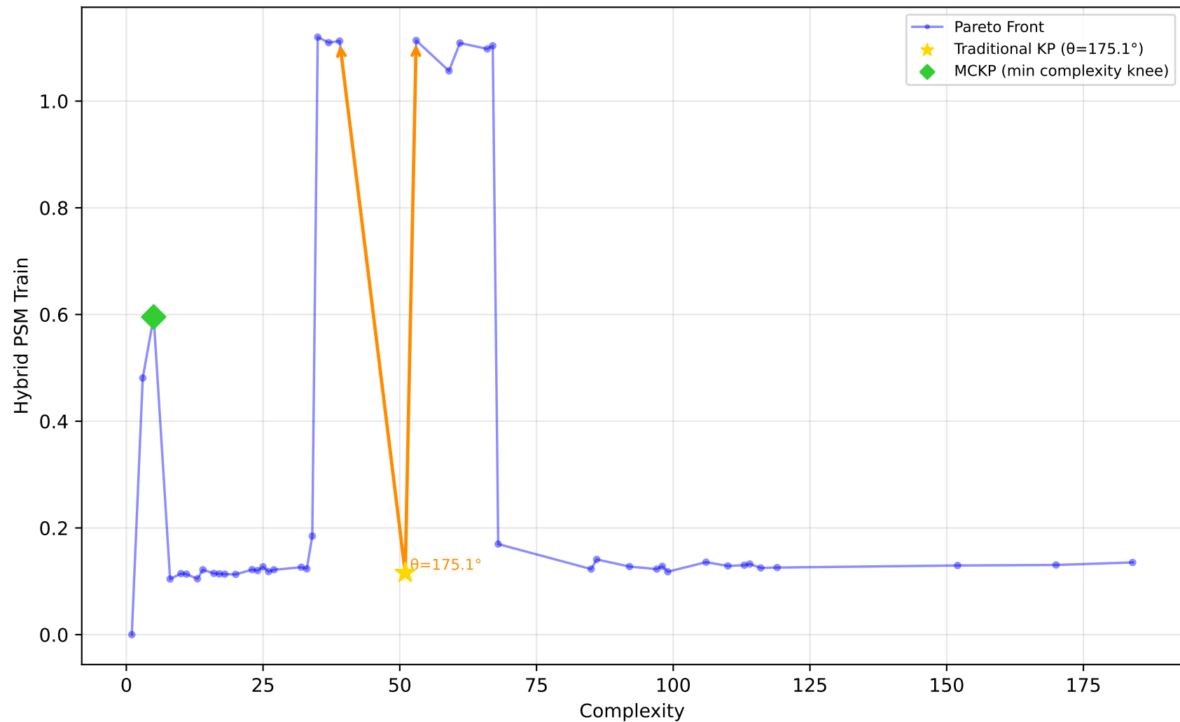
519_vinnie - Run 22 - MVP - Hybrid PSM Train \lambda_1=1.00, \lambda_2=0.00, \lambda_3=1.00 | Difficulty: 0.95 | Method: hmr
