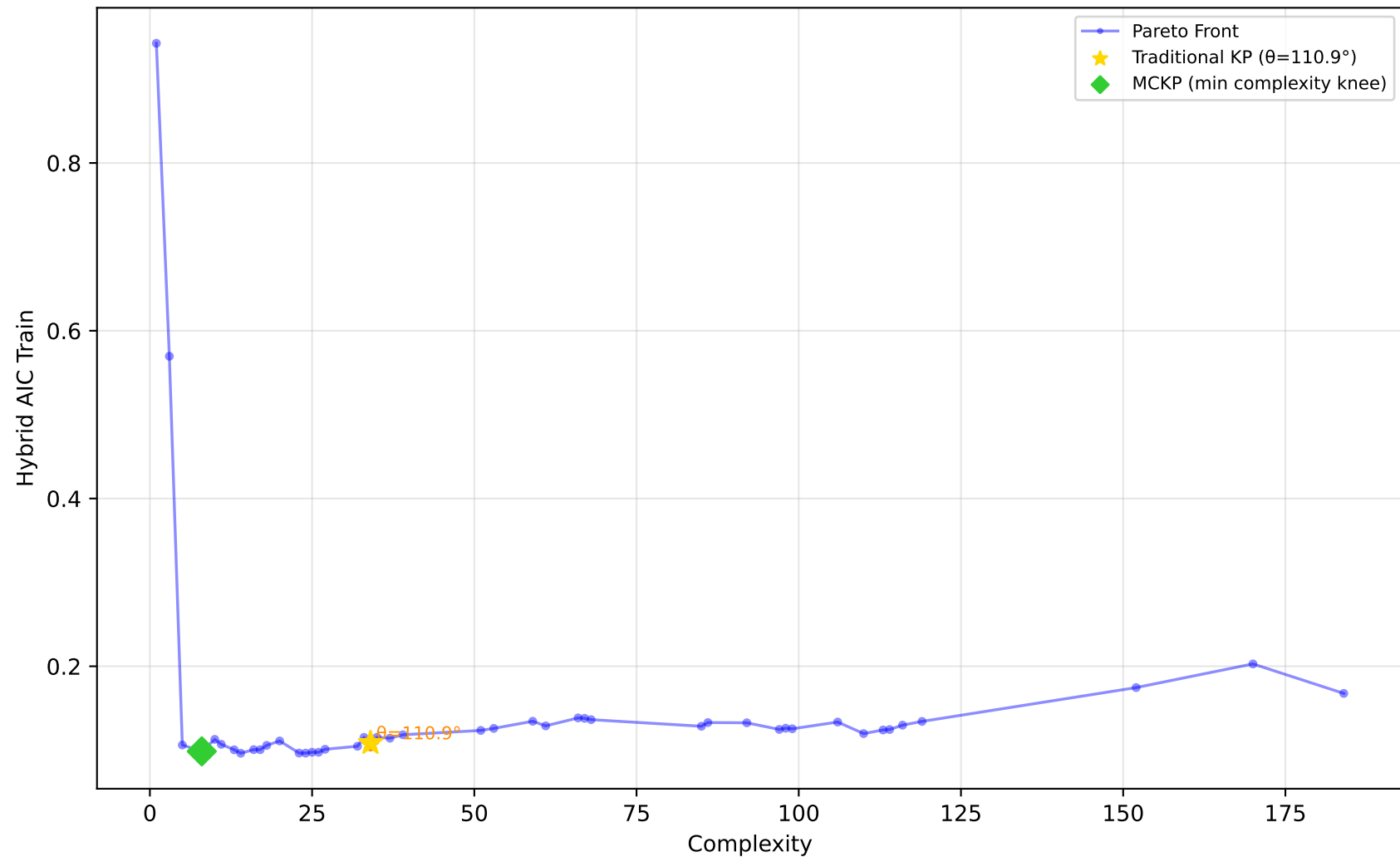
519_vinnie - Run 22 - SVP - Hybrid AIC Train \lambda_1=0.00, \lambda_2=0.00, \lambda_3=0.00 | Difficulty: 0.95 | Method: hmr
