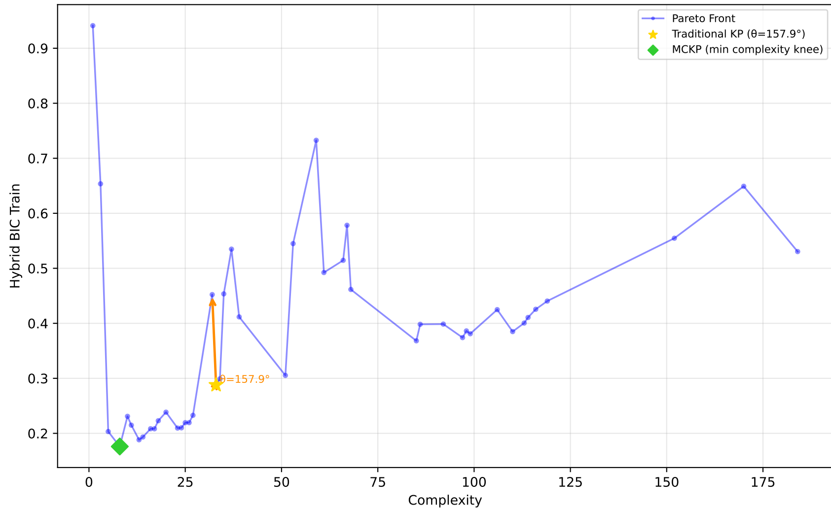
519_vinnie - Run 22 - SVP - Hybrid BIC Train \lambda_1=1.00, \lambda_2=1.00, \lambda_3=1.00 | Difficulty: 0.95 | Method: hmr
