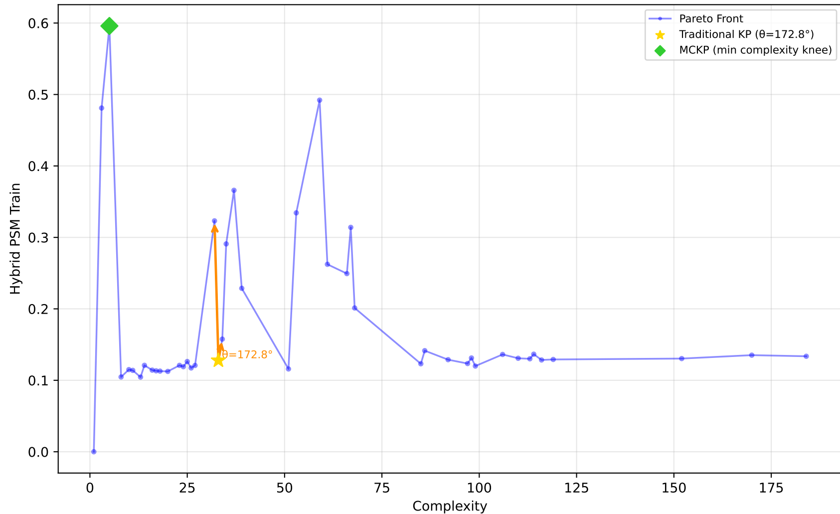
519_vinnie - Run 22 - SVP - Hybrid PSM Train \lambda_1=1.00, \lambda_2=1.00, \lambda_3=1.00 | Difficulty: 0.95 | Method: hmr
