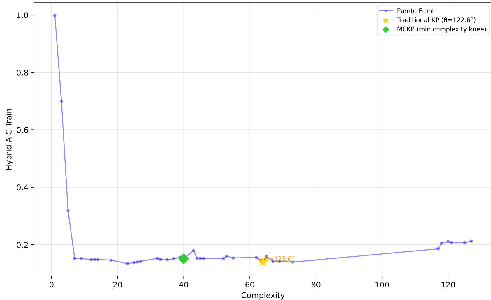
519_vinnie - Run 23 - MVP - Hybrid AIC Train \lambda_1=1.00 , \lambda_2=0.00 , \lambda_3=1.00 | Difficulty: 0.34 | Method: mckp
