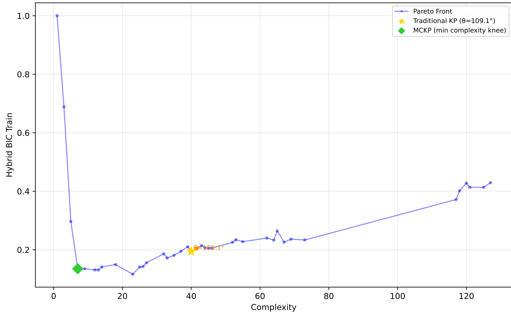
519_vinnie - Run 23 - MVP - Hybrid BIC Train \lambda_1=1.00, \lambda_2=0.00, \lambda_3=1.00 | Difficulty: 0.34 | Method: mckp
