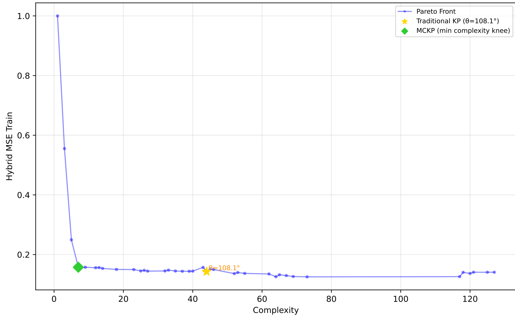
519_vinnie - Run 23 - MVP - Hybrid MSE Train \lambda_1=1.00, \lambda_2=0.00, \lambda_3=1.00 | Difficulty: 0.34 | Method: mckp
