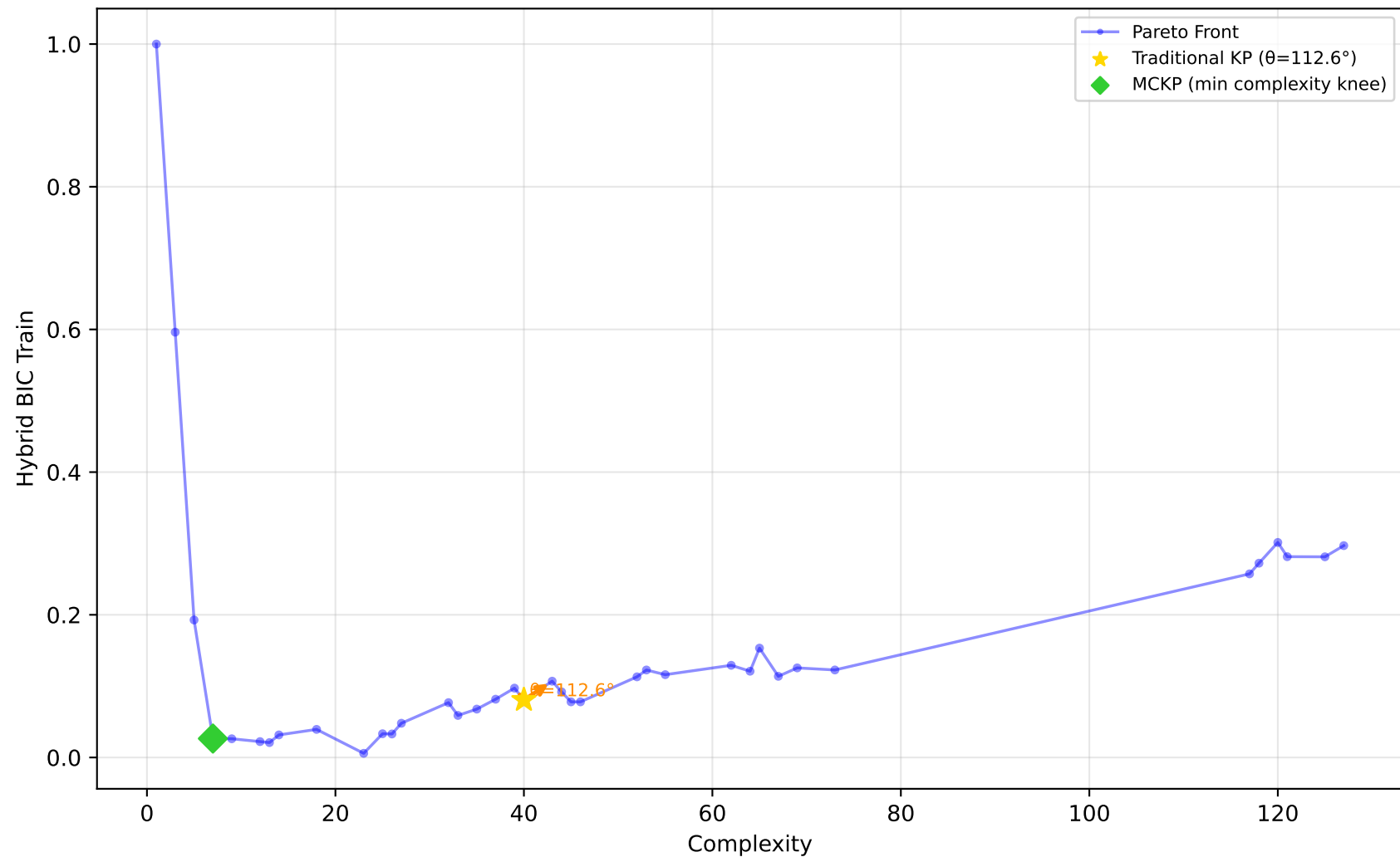
519_vinnie - Run 23 - SVP - Hybrid BIC Train \lambda_1=0.00, \lambda_2=0.00, \lambda_3=0.00 | Difficulty: 0.34 | Method: mckp
