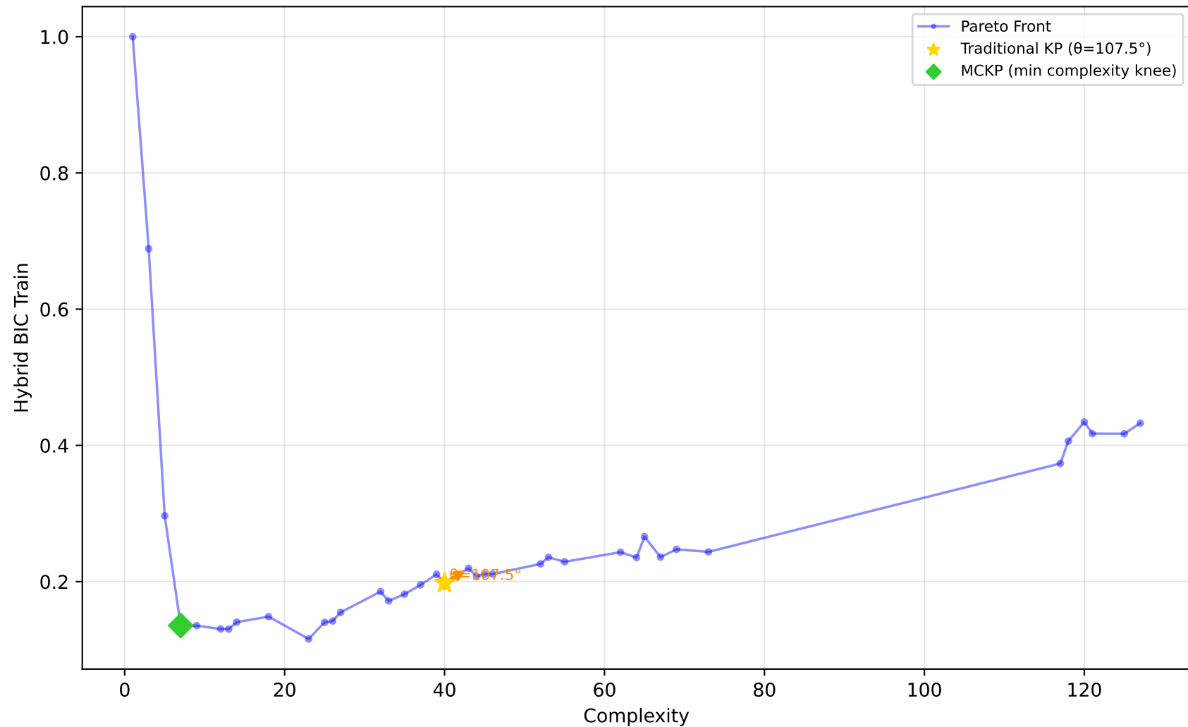
519_vinnie - Run 23 - SVP - Hybrid BIC Train \lambda_1=1.00, \lambda_2=1.00, \lambda_3=1.00 | Difficulty: 0.34 | Method: mckp
