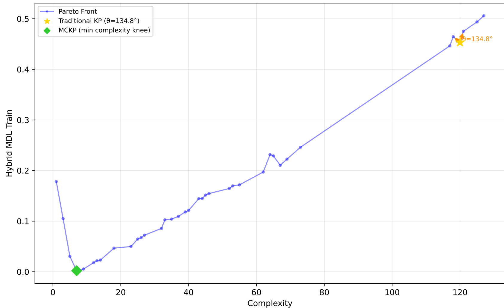
519_vinnie - Run 23 - SVP - Hybrid MDL Train \lambda_1=0.00, \lambda_2=0.00, \lambda_3=0.00 | Difficulty: 0.34 | Method: mckp
