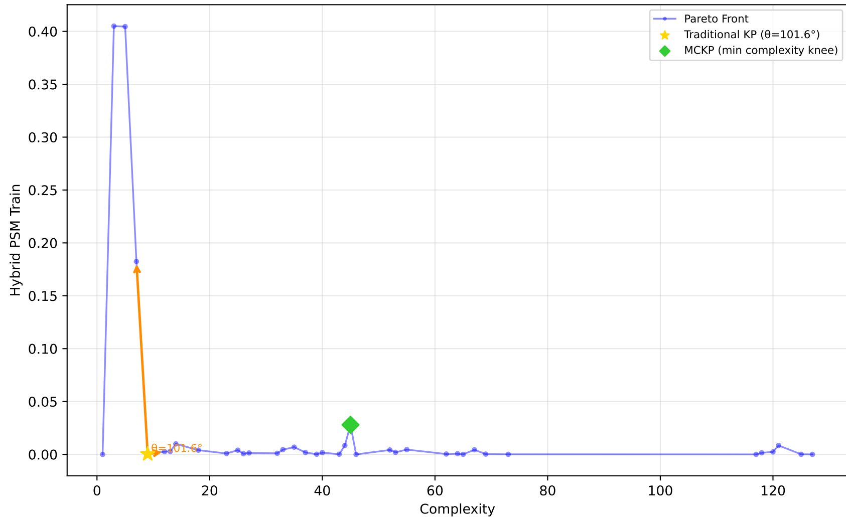
519_vinnie - Run 23 - SVP - Hybrid PSM Train \lambda_1=0.00, \lambda_2=0.00, \lambda_3=0.00 | Difficulty: 0.34 | Method: mckp
