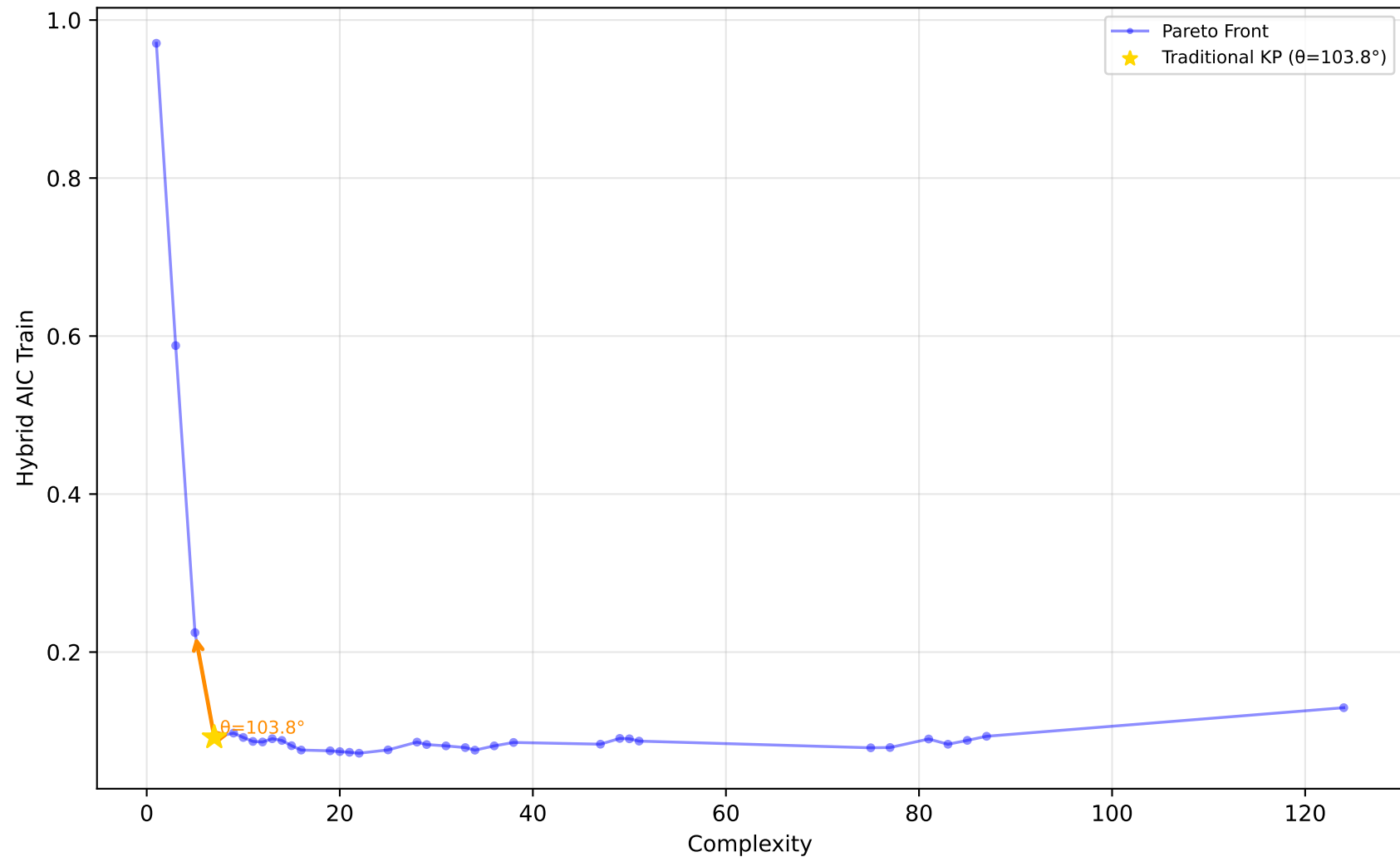
519_vinnie - Run 24 - MVP - Hybrid AIC Train \lambda_1=0.00, \lambda_2=0.10, \lambda_3=0.00 | Difficulty: 0.66 | Method: hmr
