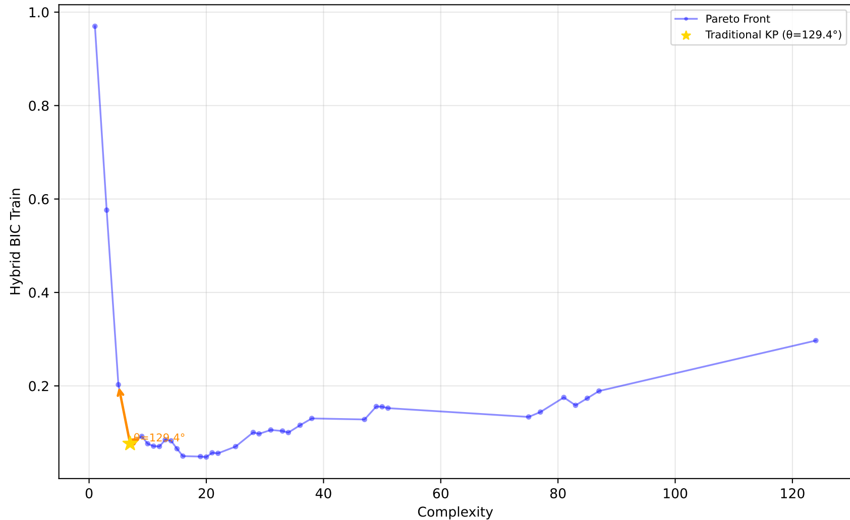
519_vinnie - Run 24 - MVP - Hybrid BIC Train \lambda_1=0.00, \lambda_2=0.10, \lambda_3=0.00 | Difficulty: 0.66 | Method: hmr
