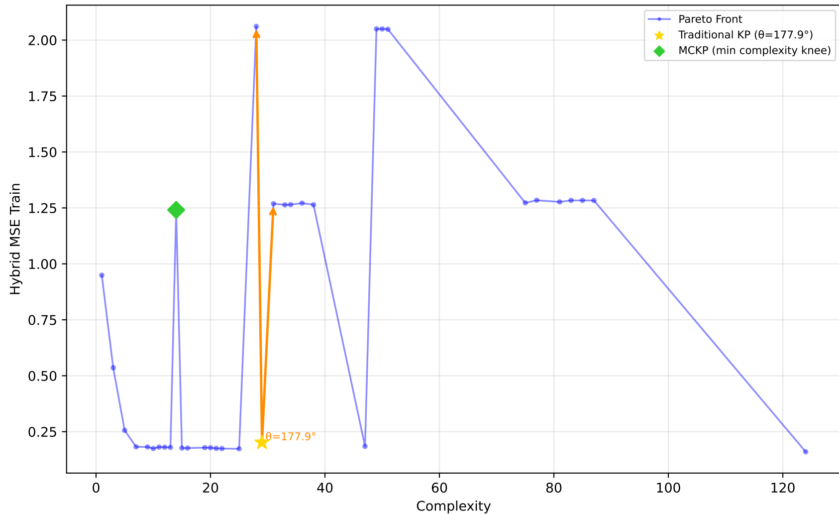
519_vinnie - Run 24 - MVP - Hybrid MSE Train \lambda_1=1.00, \lambda_2=0.00, \lambda_3=1.00 | Difficulty: 0.66 | Method: hmr
