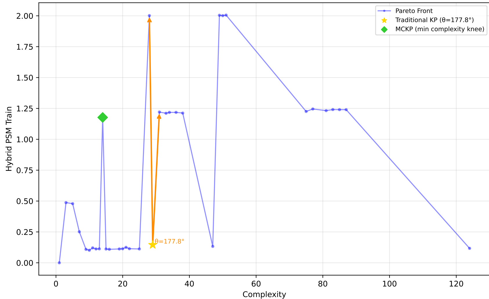
519_vinnie - Run 24 - MVP - Hybrid PSM Train \lambda_1=1.00, \lambda_2=0.00, \lambda_3=1.00 | Difficulty: 0.66 | Method: hmr
