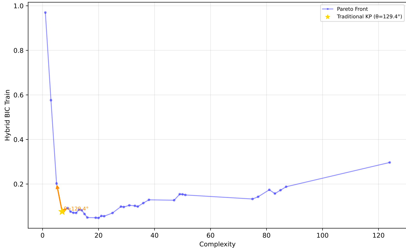
519_vinnie - Run 24 - SVP - Hybrid BIC Train \lambda_1=0.00, \lambda_2=0.00, \lambda_3=0.00 | Difficulty: 0.66 | Method: hmr
