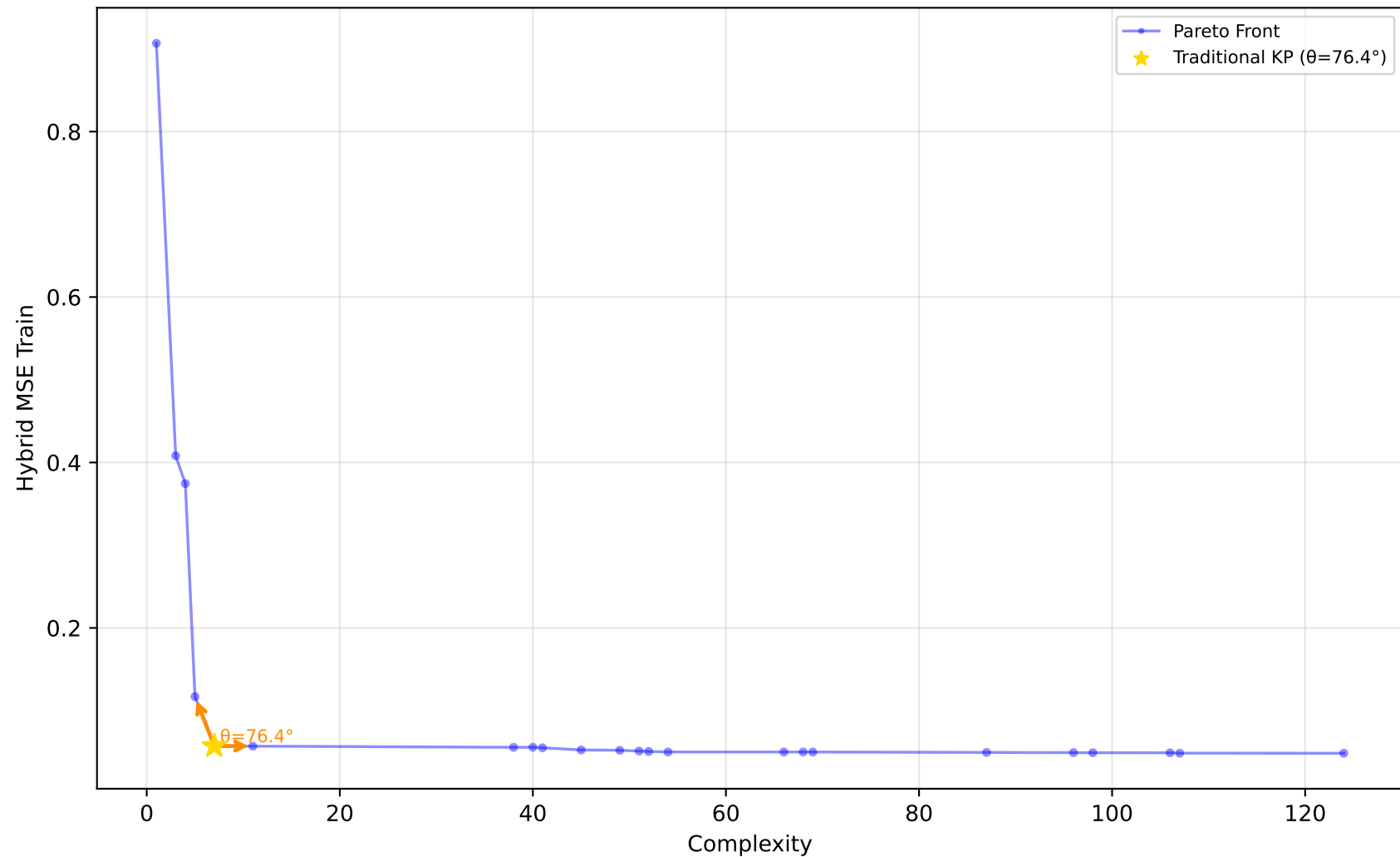
519_vinnie - Run 25 - MVP - Hybrid MSE Train \lambda_1=0.00, \lambda_2=0.10, \lambda_3=0.00 | Difficulty: 1.00 | Method: hmr
