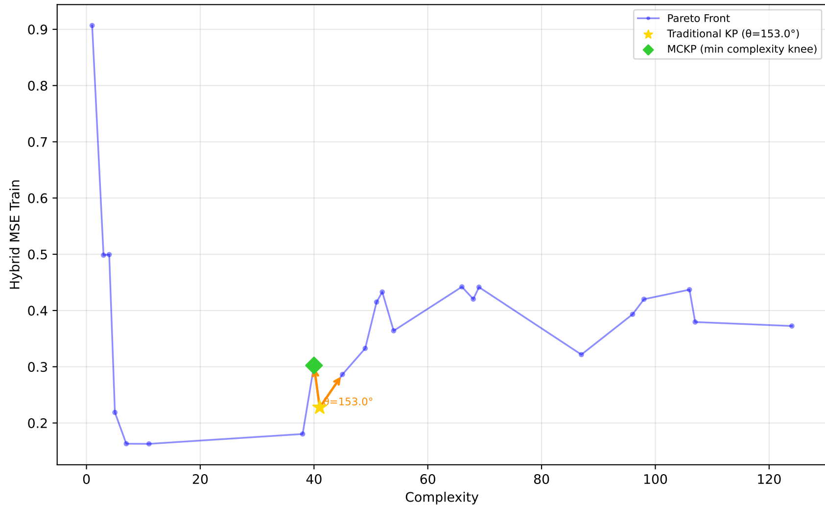
519_vinnie - Run 25 - MVP - Hybrid MSE Train \lambda_1=1.00, \lambda_2=0.00, \lambda_3=1.00 | Difficulty: 1.00 | Method: hmr
