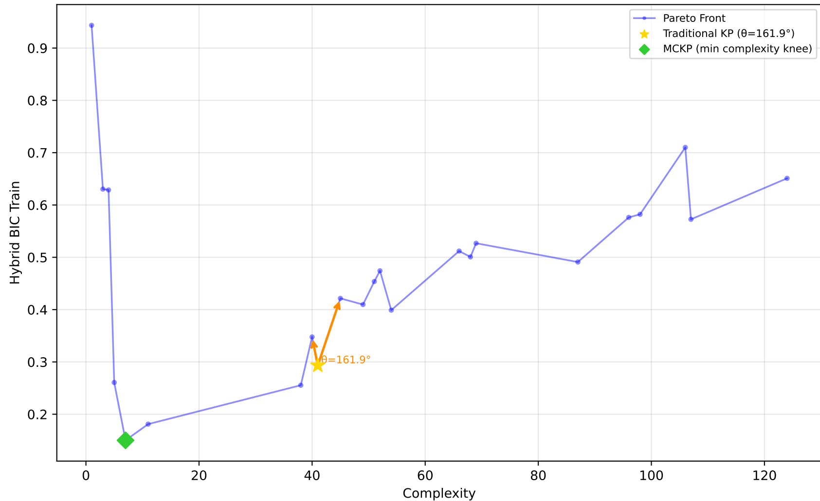
519_vinnie - Run 25 - SVP - Hybrid BIC Train \lambda_1=1.00, \lambda_2=1.00, \lambda_3=1.00 | Difficulty: 1.00 | Method: hmr
